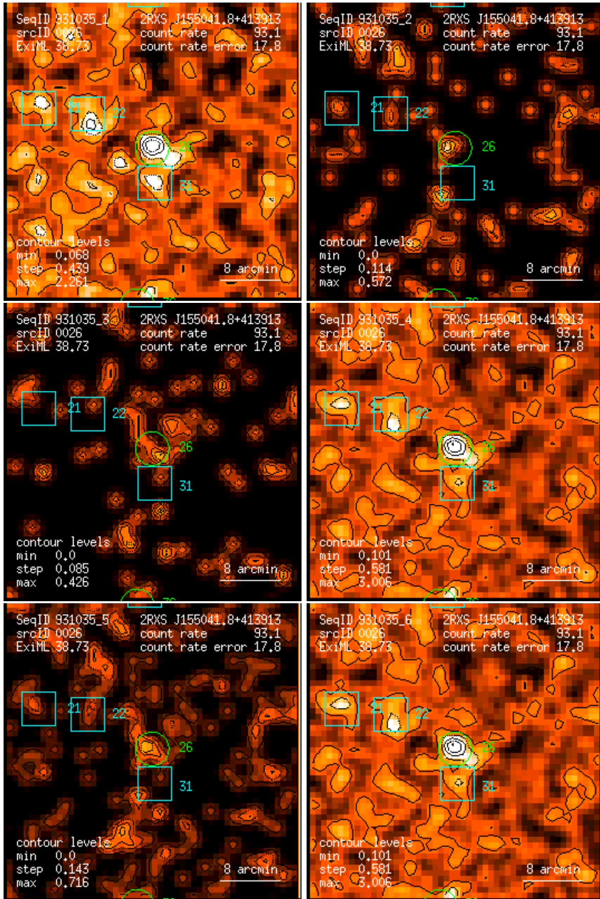
Figure 26: RASS 931035: detection 0026: band rate images, Gaussian filter: (1) PSPC channels 11 – 41, (2) 52 – 90, (3) 91 – 201, (4) 11 – 235, (5) 52 – 201, (6) 11 – 201. Broad band rates in counts/ks. Band rate contour levels in counts/ks/arcmin 2 .
