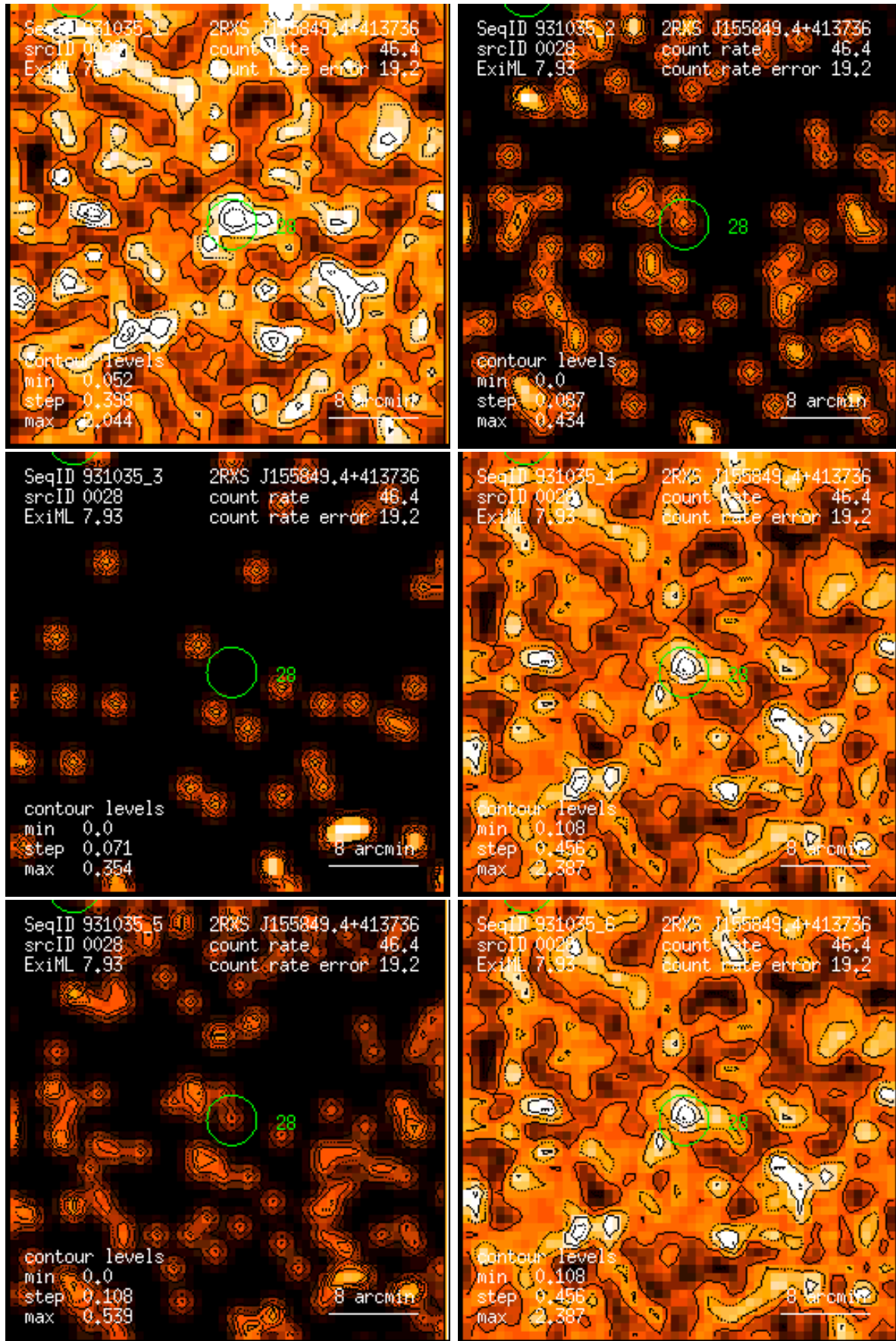
Figure 28: RASS 931035: detection 0028: band rate images, Gaussian filter: (1) PSPC channels 11 – 41, (2) 52 – 90, (3) 91 – 201, (4) 11 – 235, (5) 52 – 201, (6) 11 – 201. Broad band rates in counts/ks. Band rate contour levels in counts/ks/arcmin 2 .
