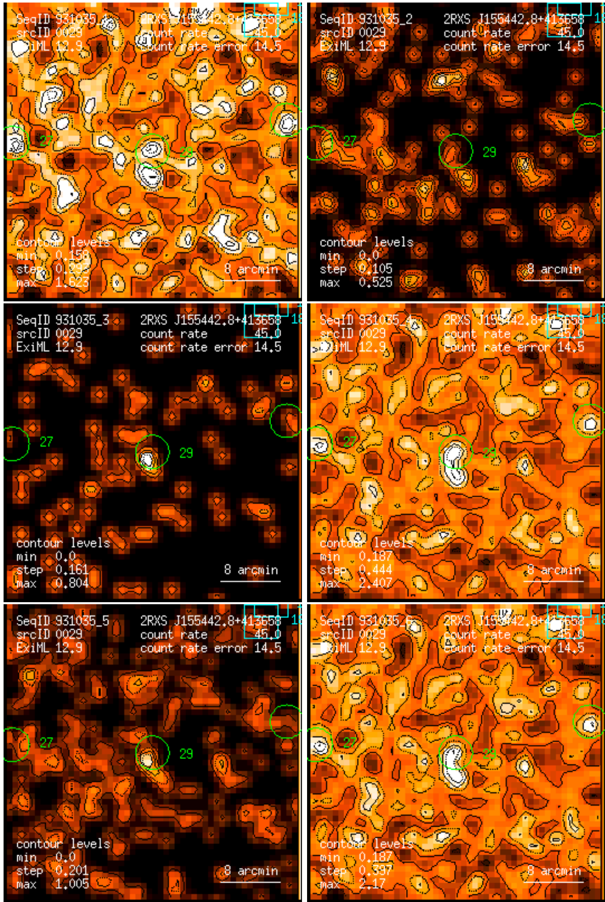
Figure 29: RASS 931035: detection 0029: band rate images, Gaussian filter: (1) PSPC channels 11 – 41, (2) 52 – 90, (3) 91 – 201, (4) 11 – 235, (5) 52 – 201, (6) 11 – 201. Broad band rates in counts/ks. Band rate contour levels in counts/ks/arcmin 2 .
