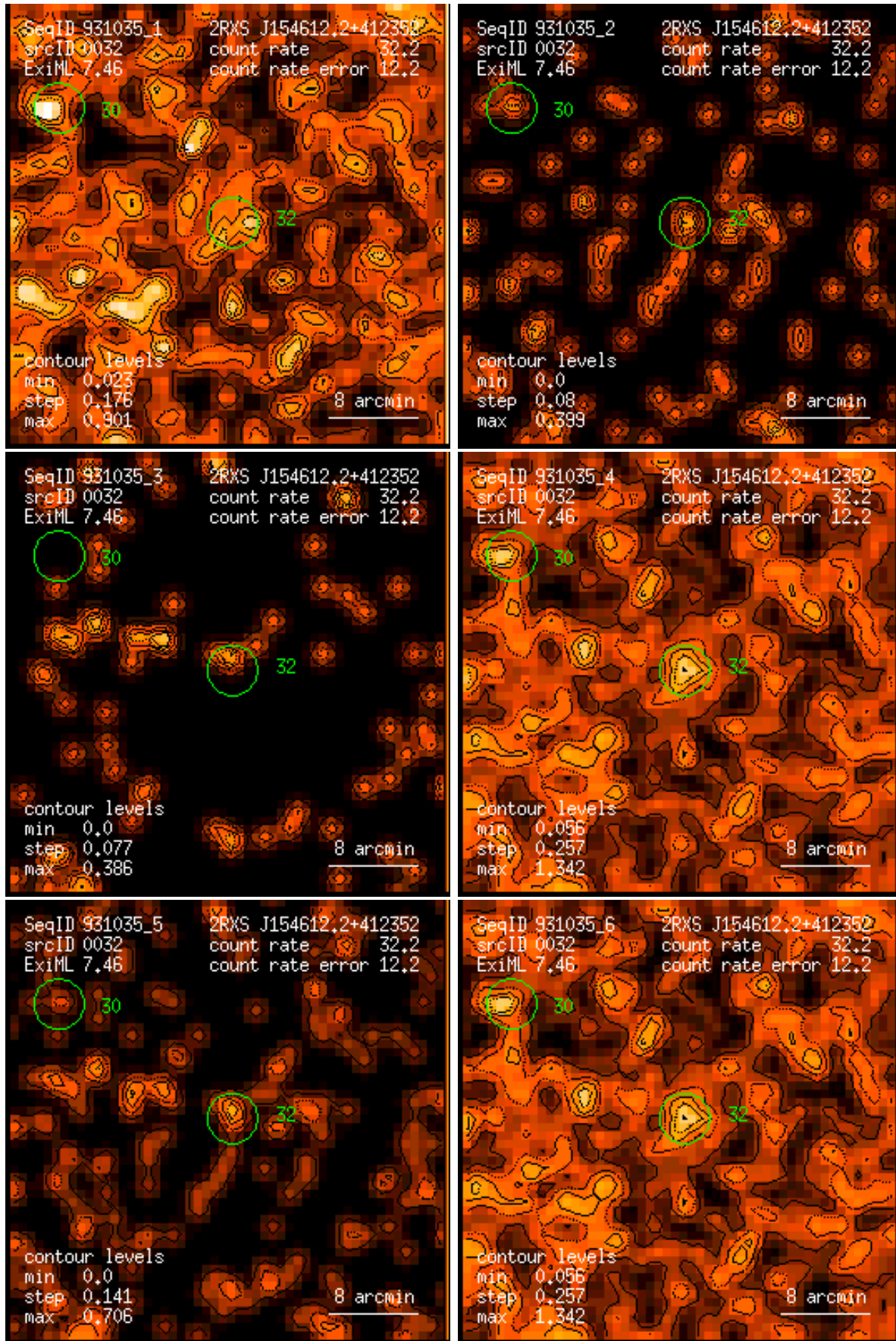
Figure 32: RASS 931035: detection 0032: band rate images, Gaussian filter: (1) PSPC channels 11 – 41, (2) 52 – 90, (3) 91 – 201, (4) 11 – 235, (5) 52 – 201, (6) 11 – 201. Broad band rates in counts/ks. Band rate contour levels in counts/ks/arcmin 2 .
