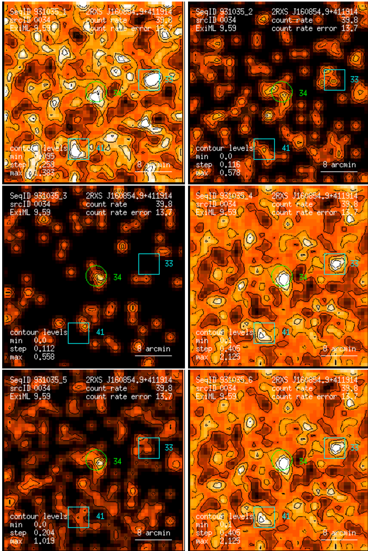
Figure 34: RASS 931035: detection 0034: band rate images, Gaussian filter: (1) PSPC channels 11 – 41, (2) 52 – 90, (3) 91 – 201, (4) 11 – 235, (5) 52 – 201, (6) 11 – 201. Broad band rates in counts/ks. Band rate contour levels in counts/ks/arcmin 2 .
