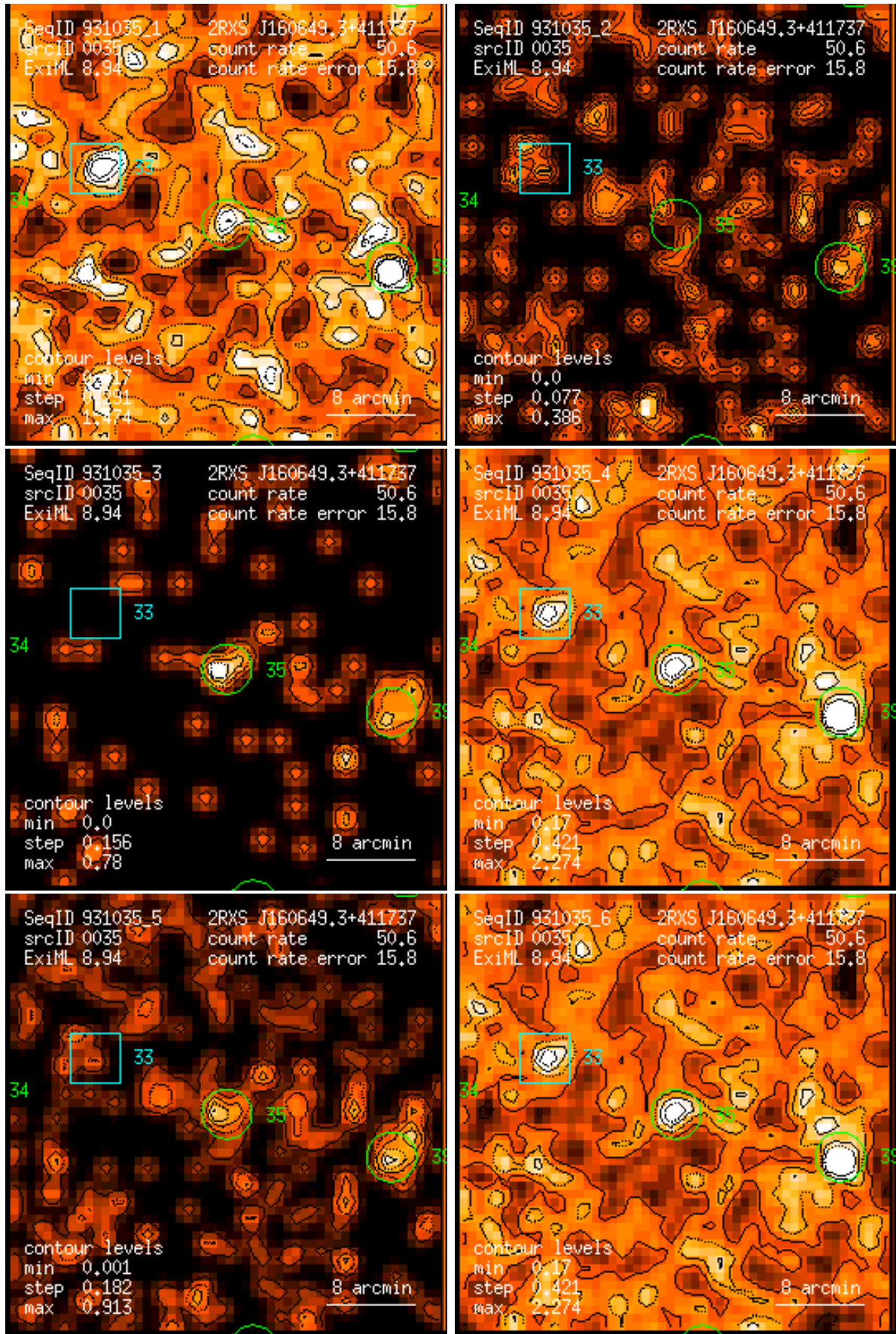
Figure 35: RASS 931035: detection 0035: band rate images, Gaussian filter: (1) PSPC channels 11 – 41, (2) 52 – 90, (3) 91 – 201, (4) 11 – 235, (5) 52 – 201, (6) 11 – 201. Broad band rates in counts/ks. Band rate contour levels in counts/ks/arcmin 2 .
