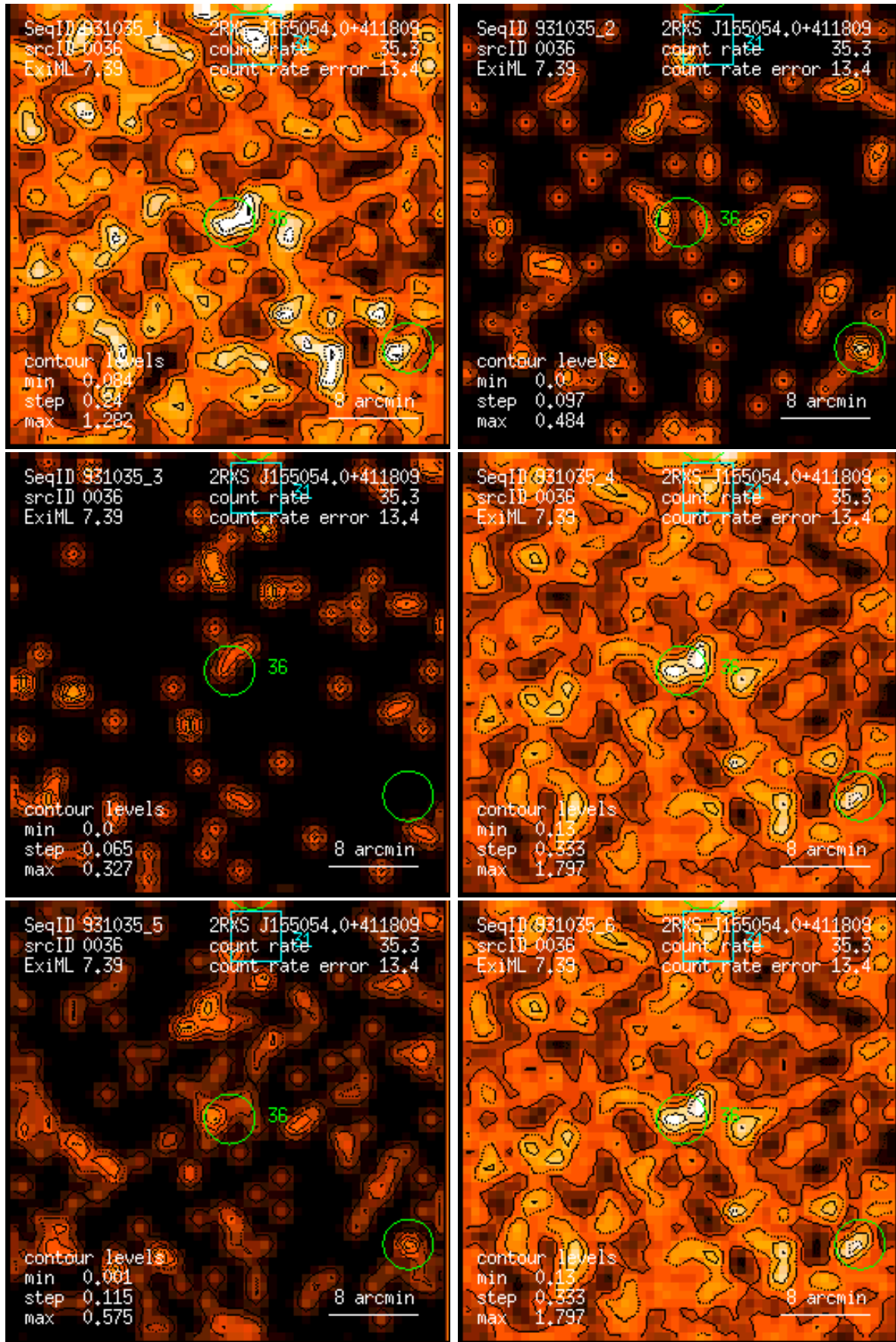
Figure 36: RASS 931035: detection 0036: band rate images, Gaussian filter: (1) PSPC channels 11 – 41, (2) 52 – 90, (3) 91 – 201, (4) 11 – 235, (5) 52 – 201, (6) 11 – 201. Broad band rates in counts/ks. Band rate contour levels in counts/ks/arcmin 2 .
