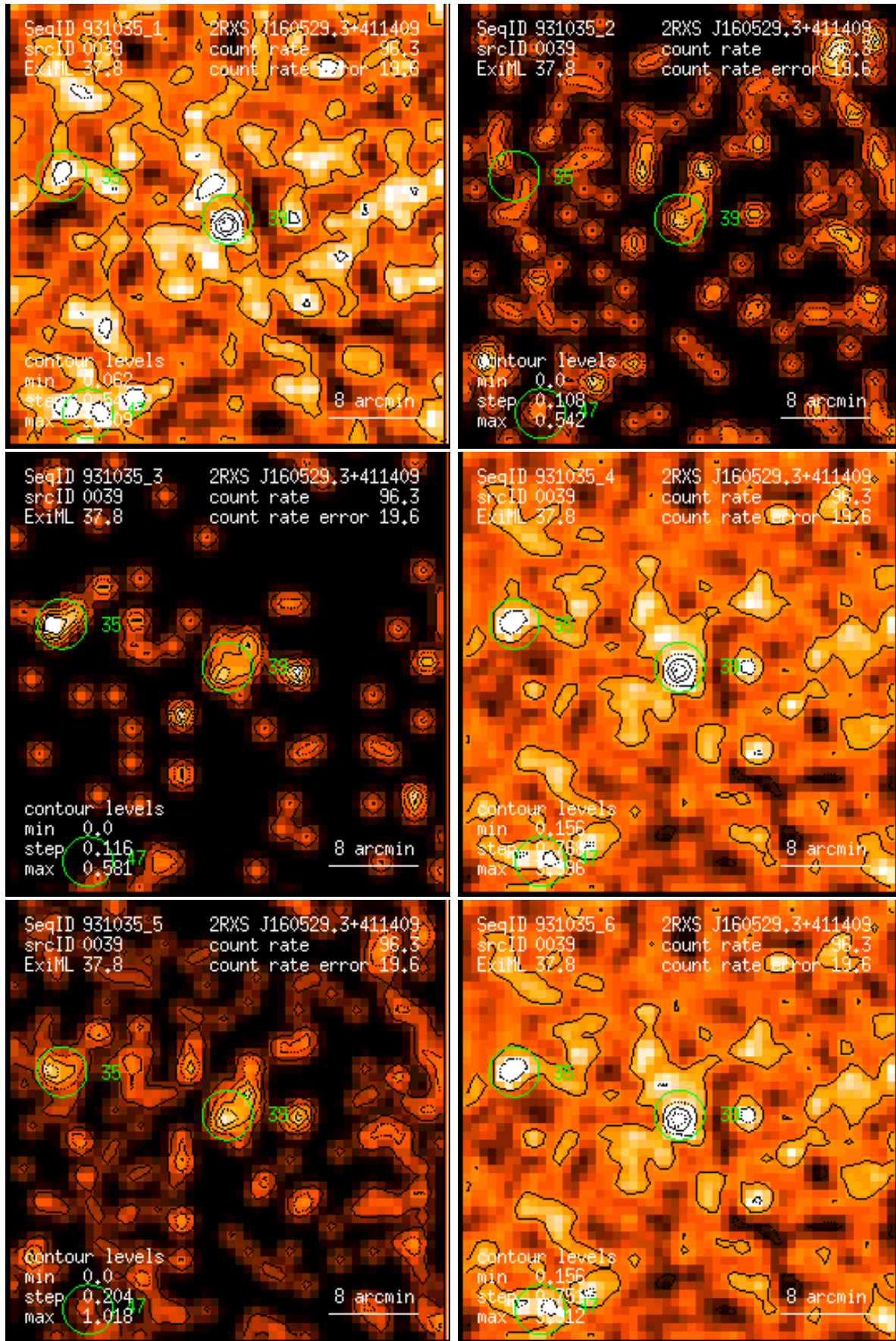
Figure 39: RASS 931035: detection 0039: band rate images, Gaussian filter: (1) PSPC channels 11 – 41, (2) 52 – 90, (3) 91 – 201, (4) 11 – 235, (5) 52 – 201, (6) 11 – 201. Broad band rates in counts/ks. Band rate contour levels in counts/ks/arcmin 2 .
