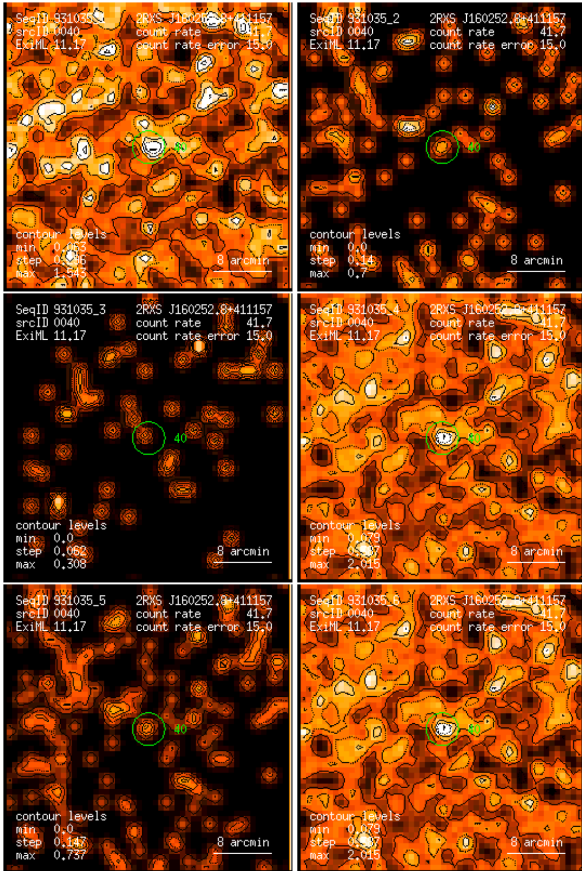
Figure 40: RASS 931035: detection 0040: band rate images, Gaussian filter: (1) PSPC channels 11 – 41, (2) 52 – 90, (3) 91 – 201, (4) 11 – 235, (5) 52 – 201, (6) 11 – 201. Broad band rates in counts/ks. Band rate contour levels in counts/ks/arcmin 2 .
