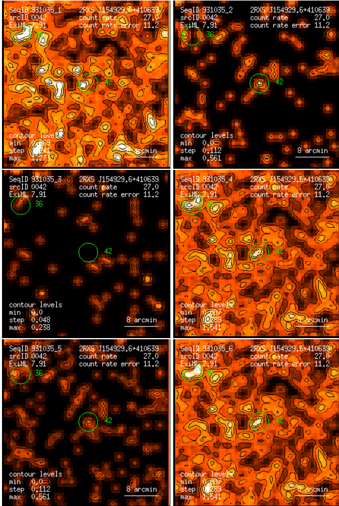
Figure 42: RASS 931035: detection 0042: band rate images, Gaussian filter: (1) PSPC channels 11 – 41, (2) 52 – 90, (3) 91 – 201, (4) 11 – 235, (5) 52 – 201, (6) 11 – 201. Broad band rates in counts/ks. Band rate contour levels in counts/ks/arcmin 2 .
