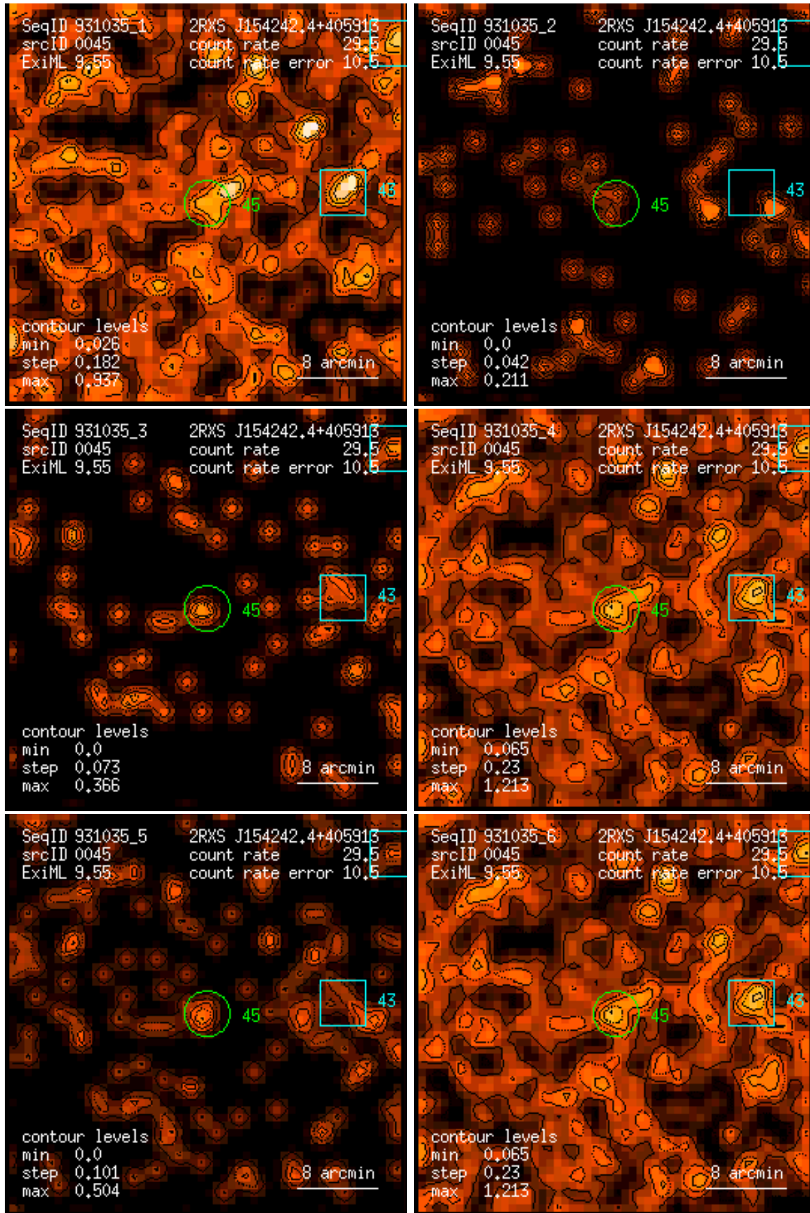
Figure 45: RASS 931035: detection 0045: band rate images, Gaussian filter: (1) PSPC channels 11 – 41, (2) 52 – 90, (3) 91 – 201, (4) 11 – 235, (5) 52 – 201, (6) 11 – 201. Broad band rates in counts/ks. Band rate contour levels in counts/ks/arcmin 2 .
