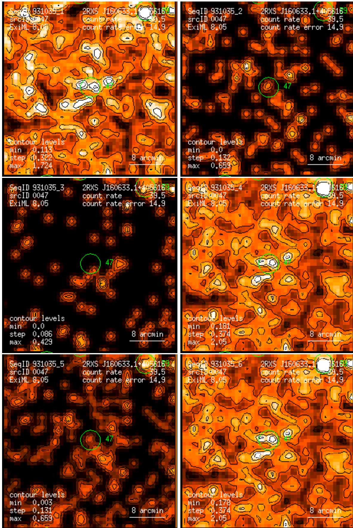
Figure 47: RASS 931035: detection 0047: band rate images, Gaussian filter: (1) PSPC channels 11 – 41, (2) 52 – 90, (3) 91 – 201, (4) 11 – 235, (5) 52 – 201, (6) 11 – 201. Broad band rates in counts/ks. Band rate contour levels in counts/ks/arcmin 2 .
