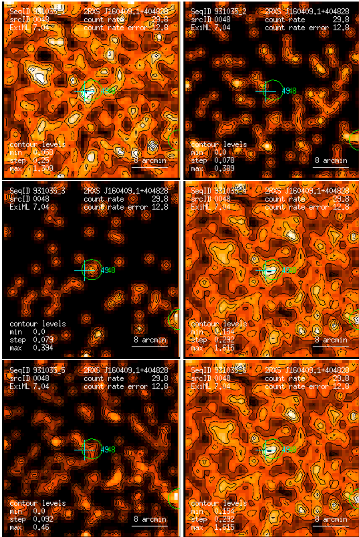
Figure 48: RASS 931035: detection 0048: band rate images, Gaussian filter: (1) PSPC channels 11 – 41, (2) 52 – 90, (3) 91 – 201, (4) 11 – 235, (5) 52 – 201, (6) 11 – 201. Broad band rates in counts/ks. Band rate contour levels in counts/ks/arcmin 2 .
