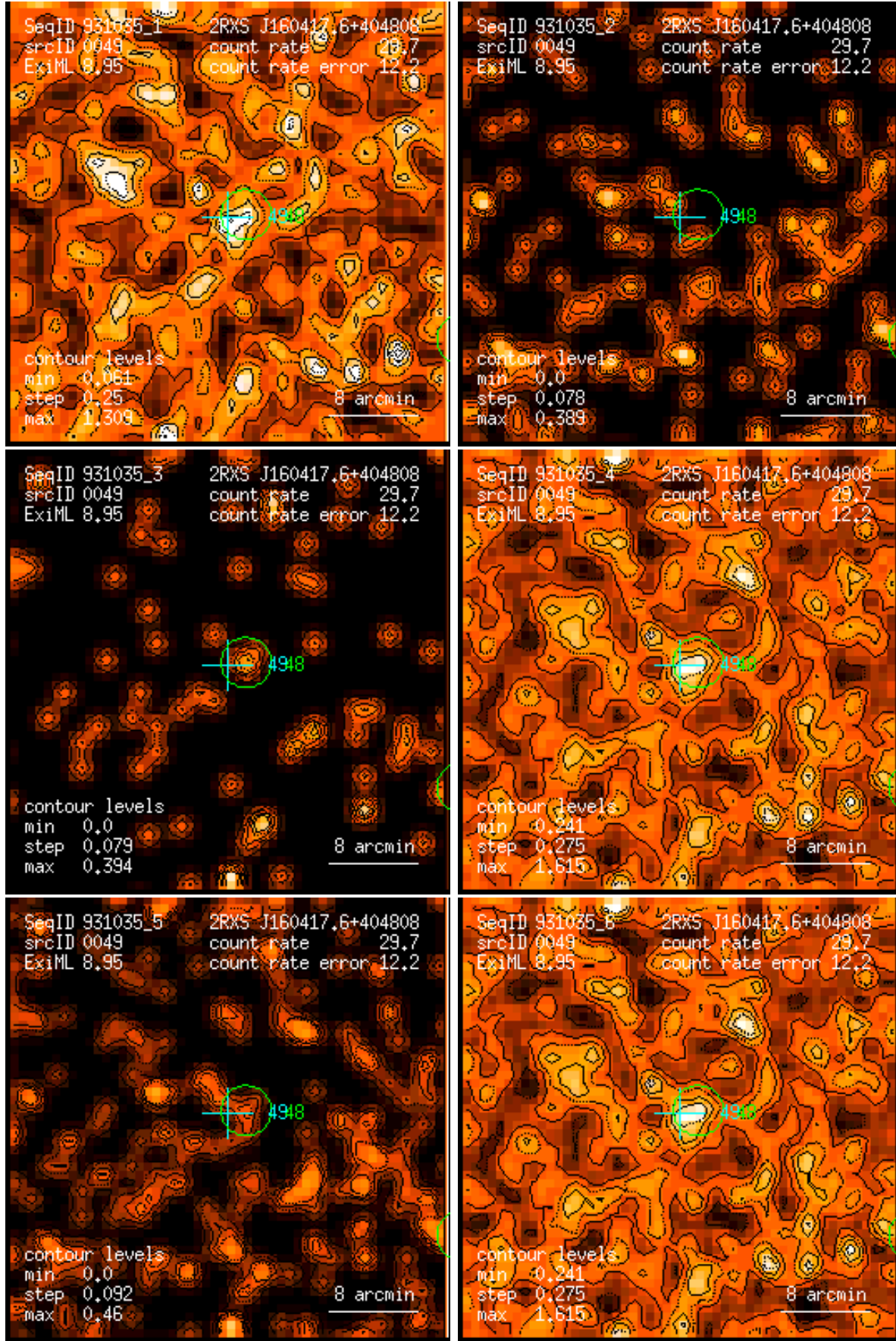
Figure 49: RASS 931035: detection 0049: band rate images, Gaussian filter: (1) PSPC channels 11 – 41, (2) 52 – 90, (3) 91 – 201, (4) 11 – 235, (5) 52 – 201, (6) 11 – 201. Broad band rates in counts/ks. Band rate contour levels in counts/ks/arcmin 2 .
