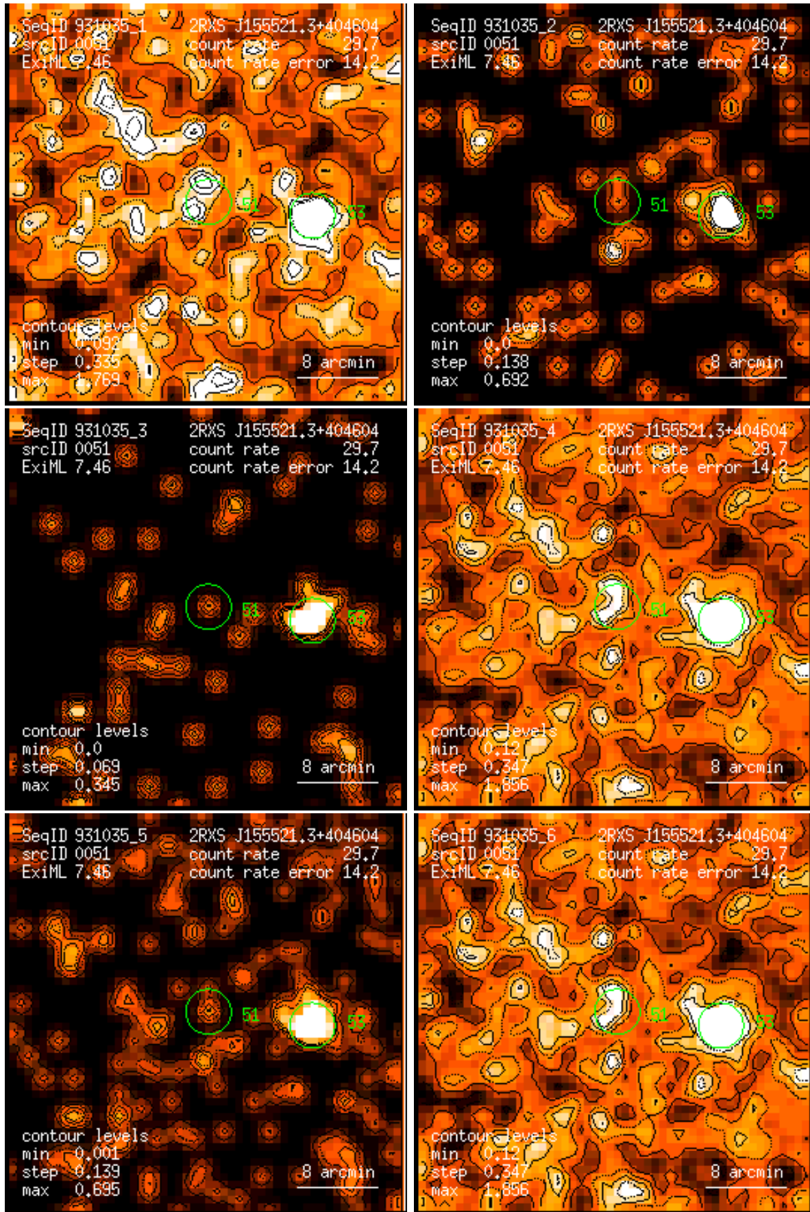
Figure 51: RASS 931035: detection 0051: band rate images, Gaussian filter: (1) PSPC channels 11 – 41, (2) 52 – 90, (3) 91 – 201, (4) 11 – 235, (5) 52 – 201, (6) 11 – 201. Broad band rates in counts/ks. Band rate contour levels in counts/ks/arcmin 2 .
