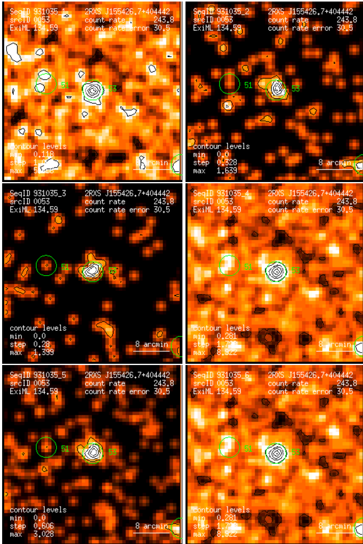
Figure 53: RASS 931035: detection 0053: band rate images, Gaussian filter: (1) PSPC channels 11 – 41, (2) 52 – 90, (3) 91 – 201, (4) 11 – 235, (5) 52 – 201, (6) 11 – 201. Broad band rates in counts/ks. Band rate contour levels in counts/ks/arcmin 2 .
