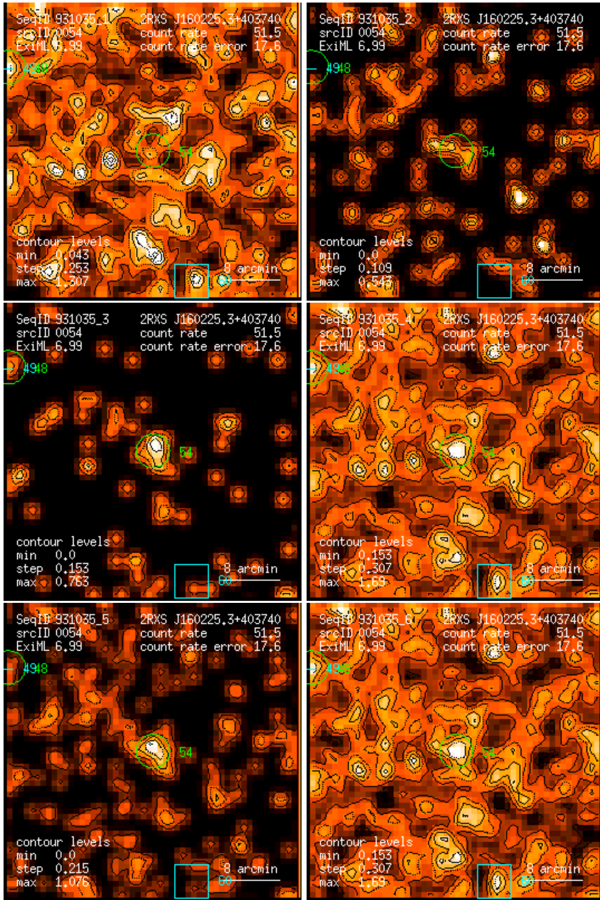
Figure 54: RASS 931035: detection 0054: band rate images, Gaussian filter: (1) PSPC channels 11 – 41, (2) 52 – 90, (3) 91 – 201, (4) 11 – 235, (5) 52 – 201, (6) 11 – 201. Broad band rates in counts/ks. Band rate contour levels in counts/ks/arcmin 2 .
