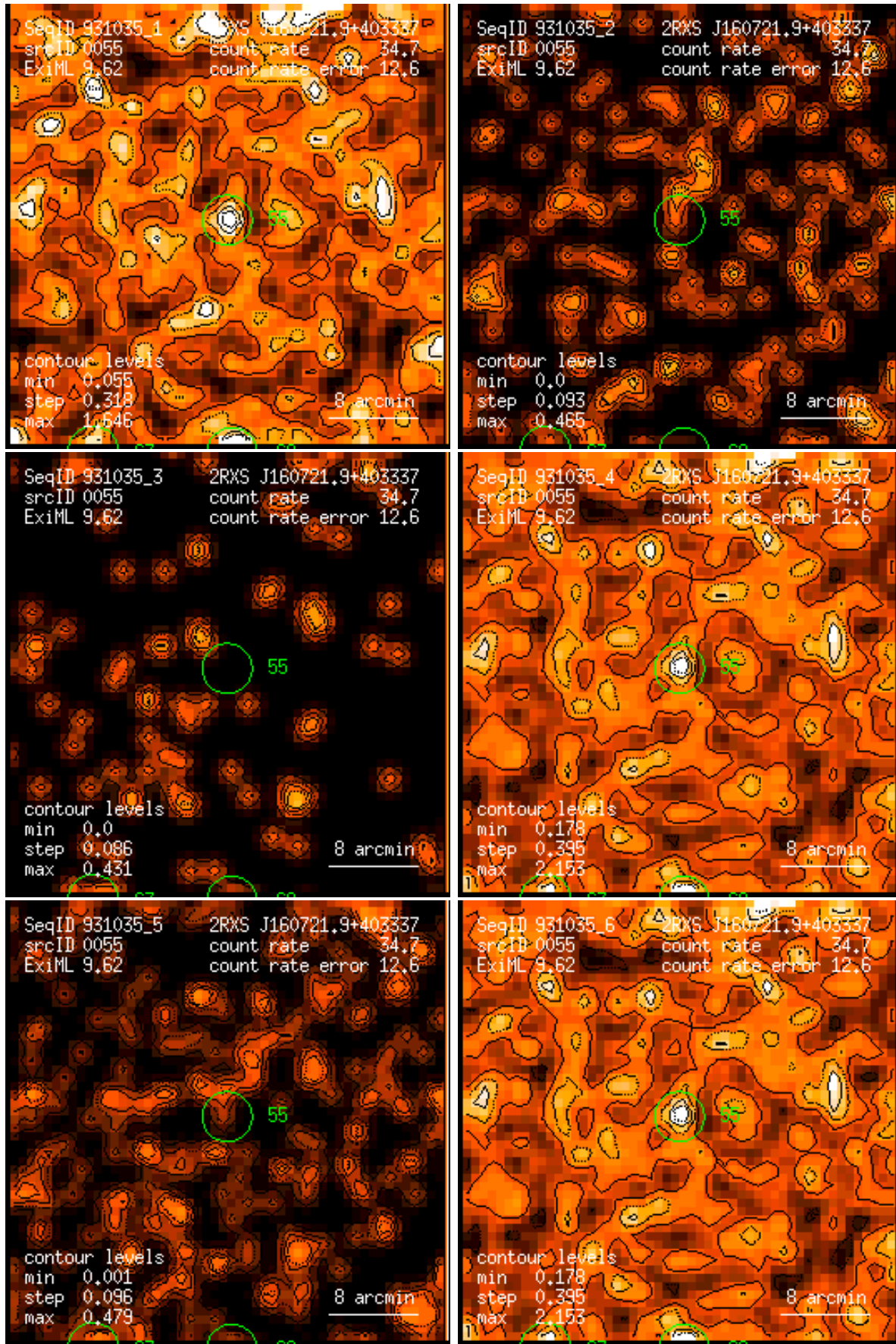
Figure 55: RASS 931035: detection 0055: band rate images, Gaussian filter: (1) PSPC channels 11 – 41, (2) 52 – 90, (3) 91 – 201, (4) 11 – 235, (5) 52 – 201, (6) 11 – 201. Broad band rates in counts/ks. Band rate contour levels in counts/ks/arcmin 2 .
