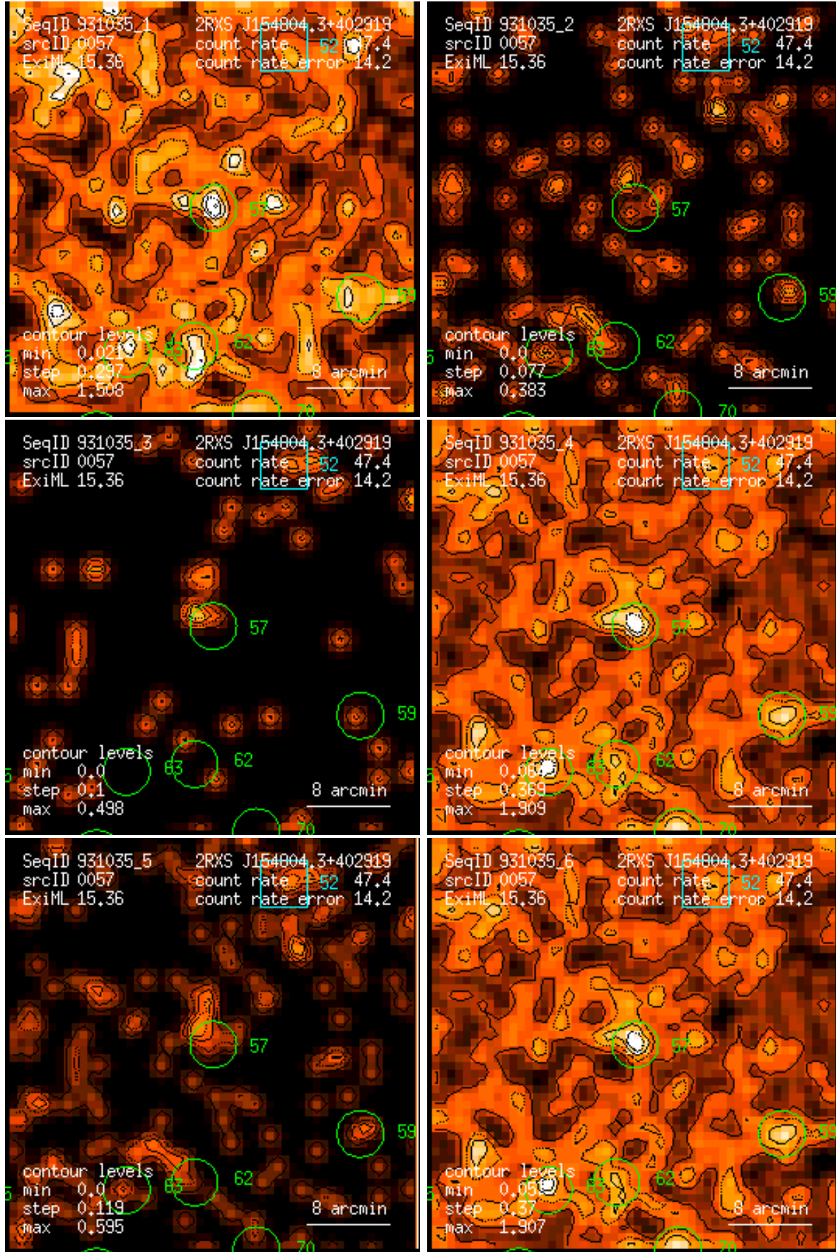
Figure 57: RASS 931035: detection 0057: band rate images, Gaussian filter: (1) PSPC channels 11 – 41, (2) 52 – 90, (3) 91 – 201, (4) 11 – 235, (5) 52 – 201, (6) 11 – 201. Broad band rates in counts/ks. Band rate contour levels in counts/ks/arcmin 2 .
