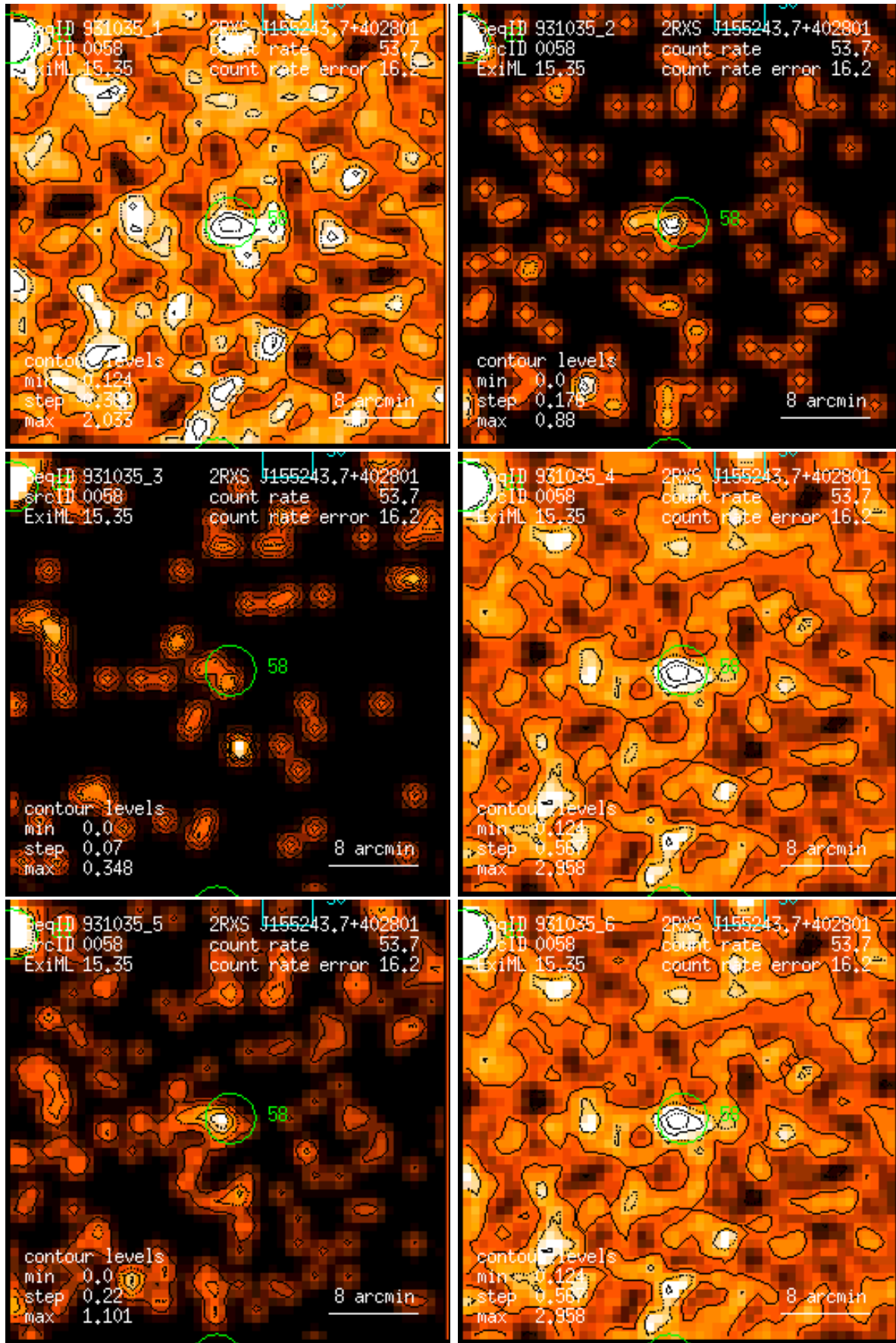
Figure 58: RASS 931035: detection 0058: band rate images, Gaussian filter: (1) PSPC channels 11 – 41, (2) 52 – 90, (3) 91 – 201, (4) 11 – 235, (5) 52 – 201, (6) 11 – 201. Broad band rates in counts/ks. Band rate contour levels in counts/ks/arcmin 2 .
