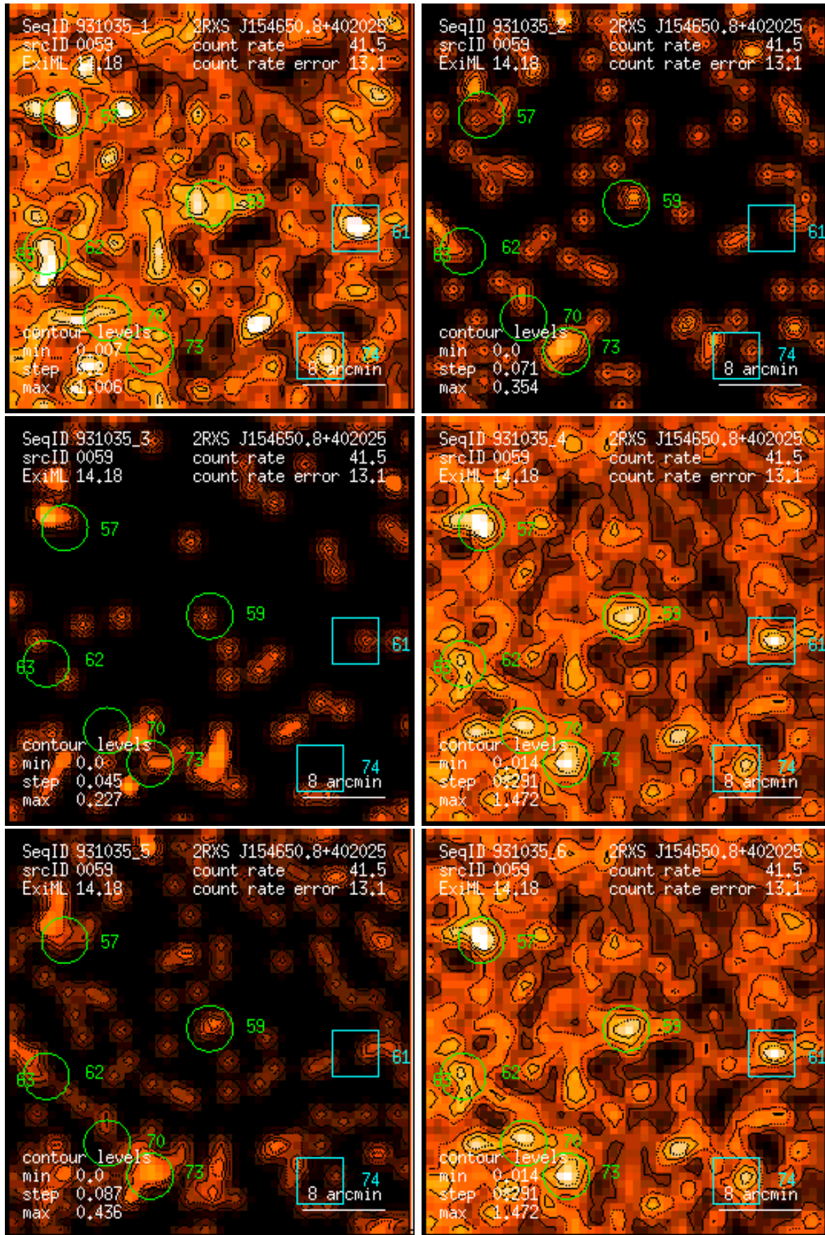
Figure 59: RASS 931035: detection 0059: band rate images, Gaussian filter: (1) PSPC channels 11 – 41, (2) 52 – 90, (3) 91 – 201, (4) 11 – 235, (5) 52 – 201, (6) 11 – 201. Broad band rates in counts/ks. Band rate contour levels in counts/ks/arcmin 2 .
