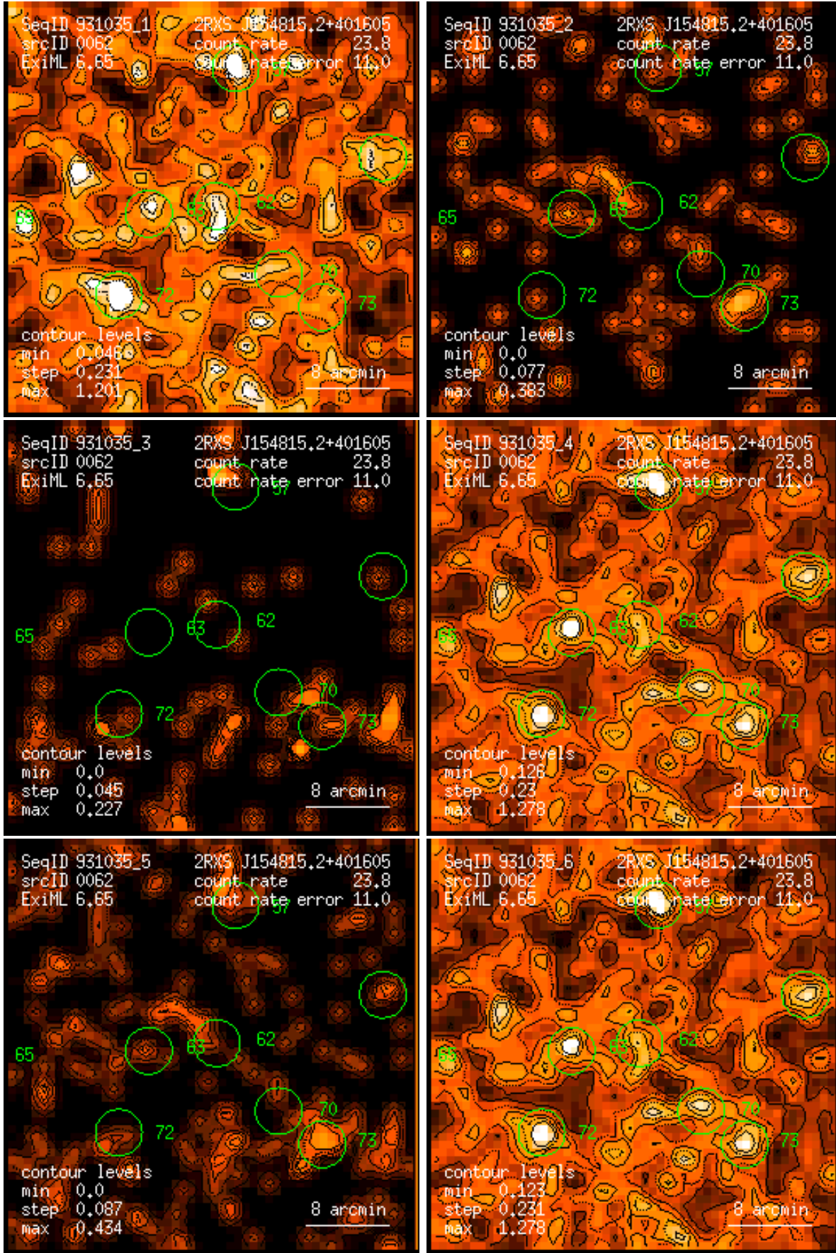
Figure 62: RASS 931035: detection 0062: band rate images, Gaussian filter: (1) PSPC channels 11 – 41, (2) 52 – 90, (3) 91 – 201, (4) 11 – 235, (5) 52 – 201, (6) 11 – 201. Broad band rates in counts/ks. Band rate contour levels in counts/ks/arcmin 2 .
