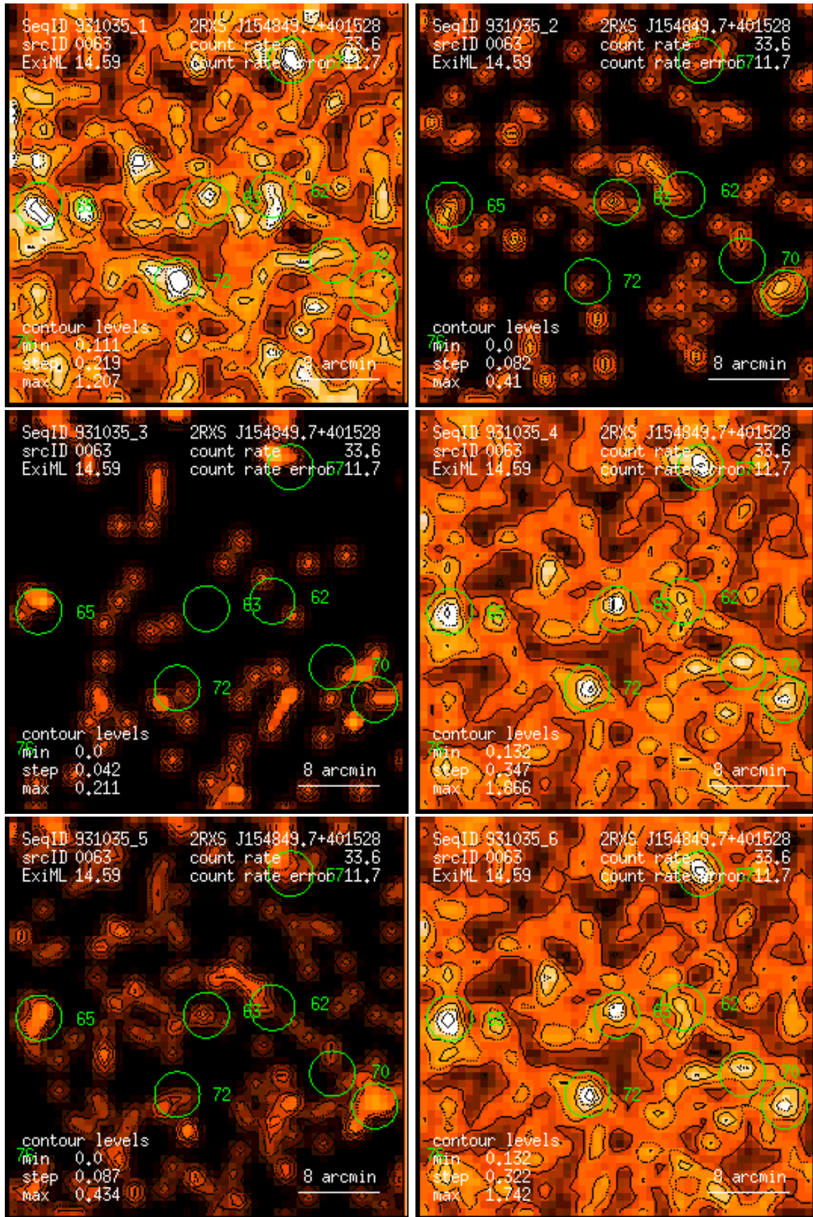
Figure 63: RASS 931035: detection 0063: band rate images, Gaussian filter: (1) PSPC channels 11 – 41, (2) 52 – 90, (3) 91 – 201, (4) 11 – 235, (5) 52 – 201, (6) 11 – 201. Broad band rates in counts/ks. Band rate contour levels in counts/ks/arcmin 2 .
