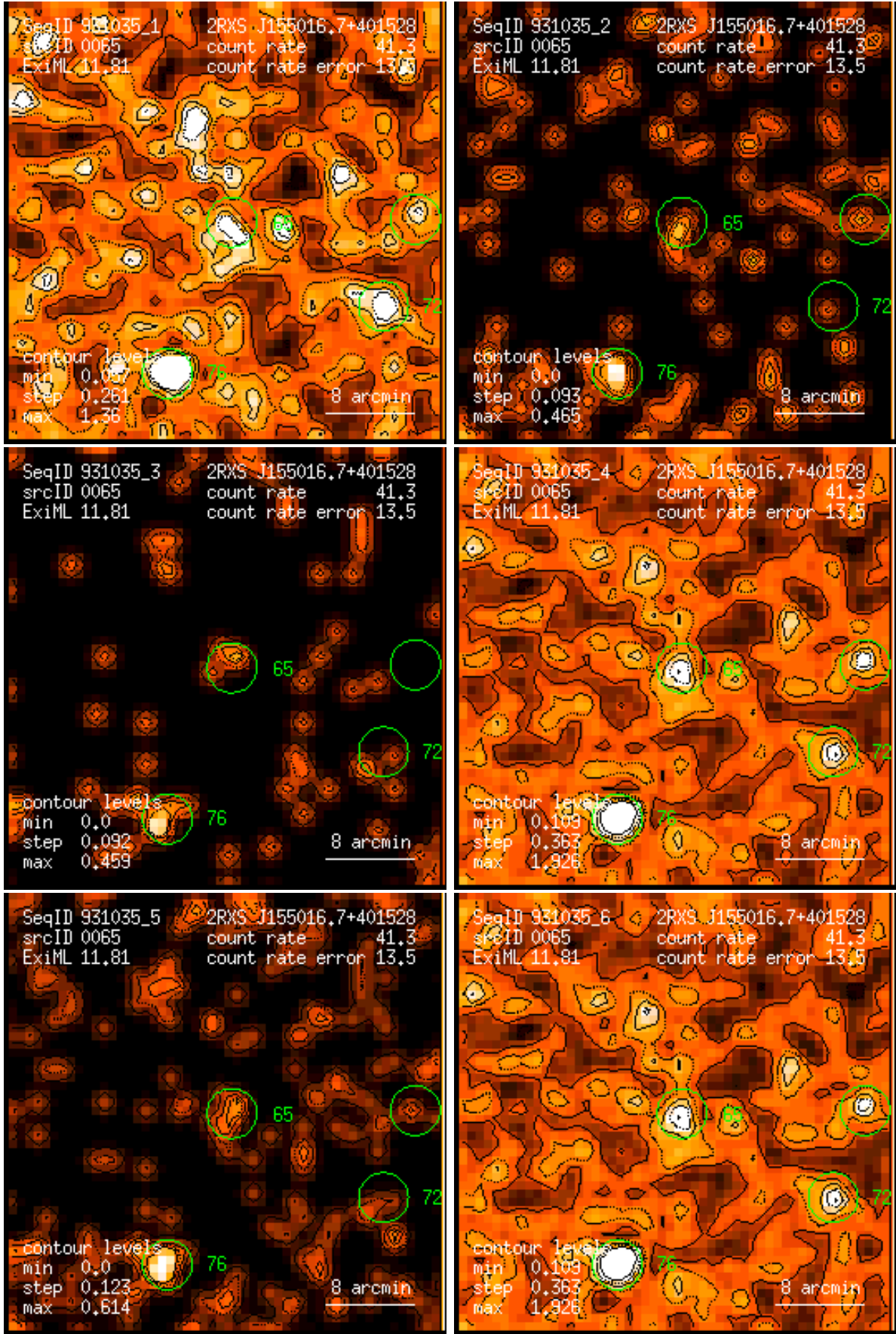
Figure 65: RASS 931035: detection 0065: band rate images, Gaussian filter: (1) PSPC channels 11 – 41, (2) 52 – 90, (3) 91 – 201, (4) 11 – 235, (5) 52 – 201, (6) 11 – 201. Broad band rates in counts/ks. Band rate contour levels in counts/ks/arcmin 2 .
