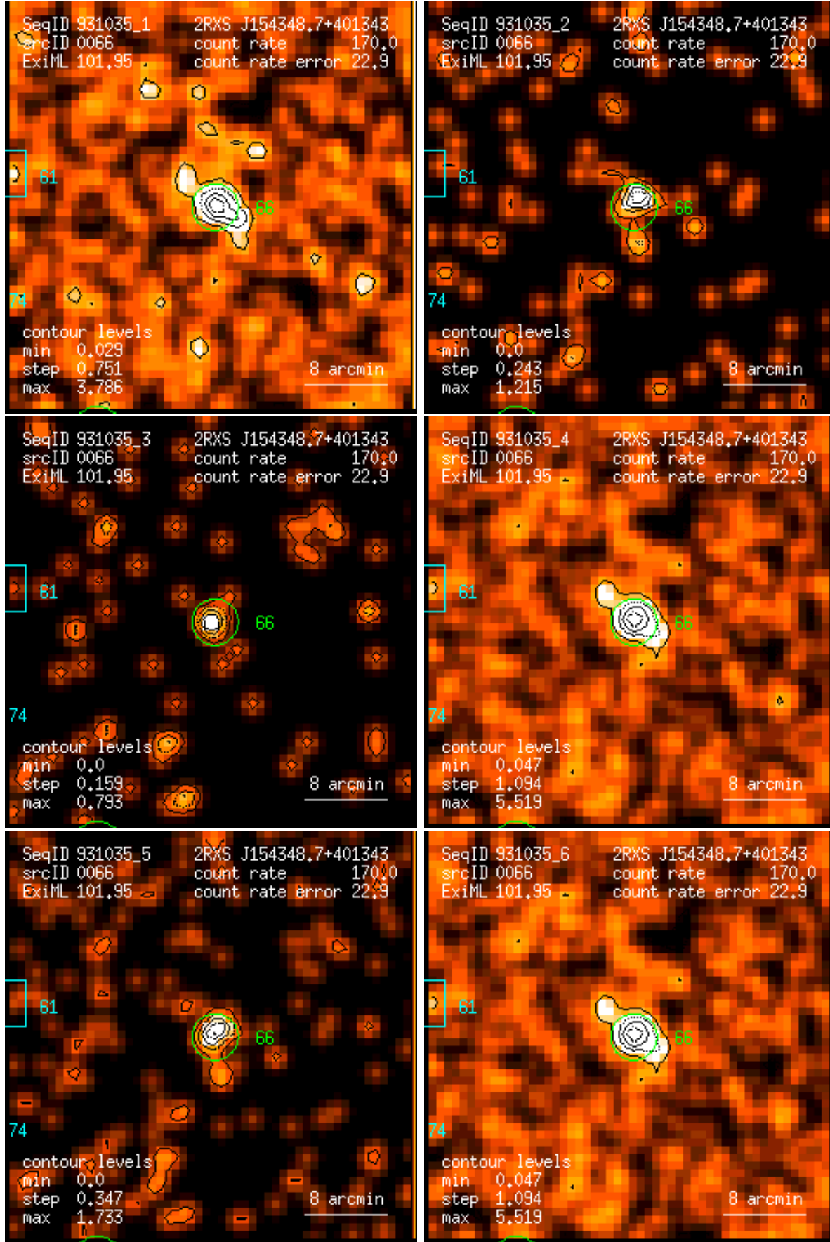
Figure 66: RASS 931035: detection 0066: band rate images, Gaussian filter: (1) PSPC channels 11 – 41, (2) 52 – 90, (3) 91 – 201, (4) 11 – 235, (5) 52 – 201, (6) 11 – 201. Broad band rates in counts/ks. Band rate contour levels in counts/ks/arcmin 2 .
