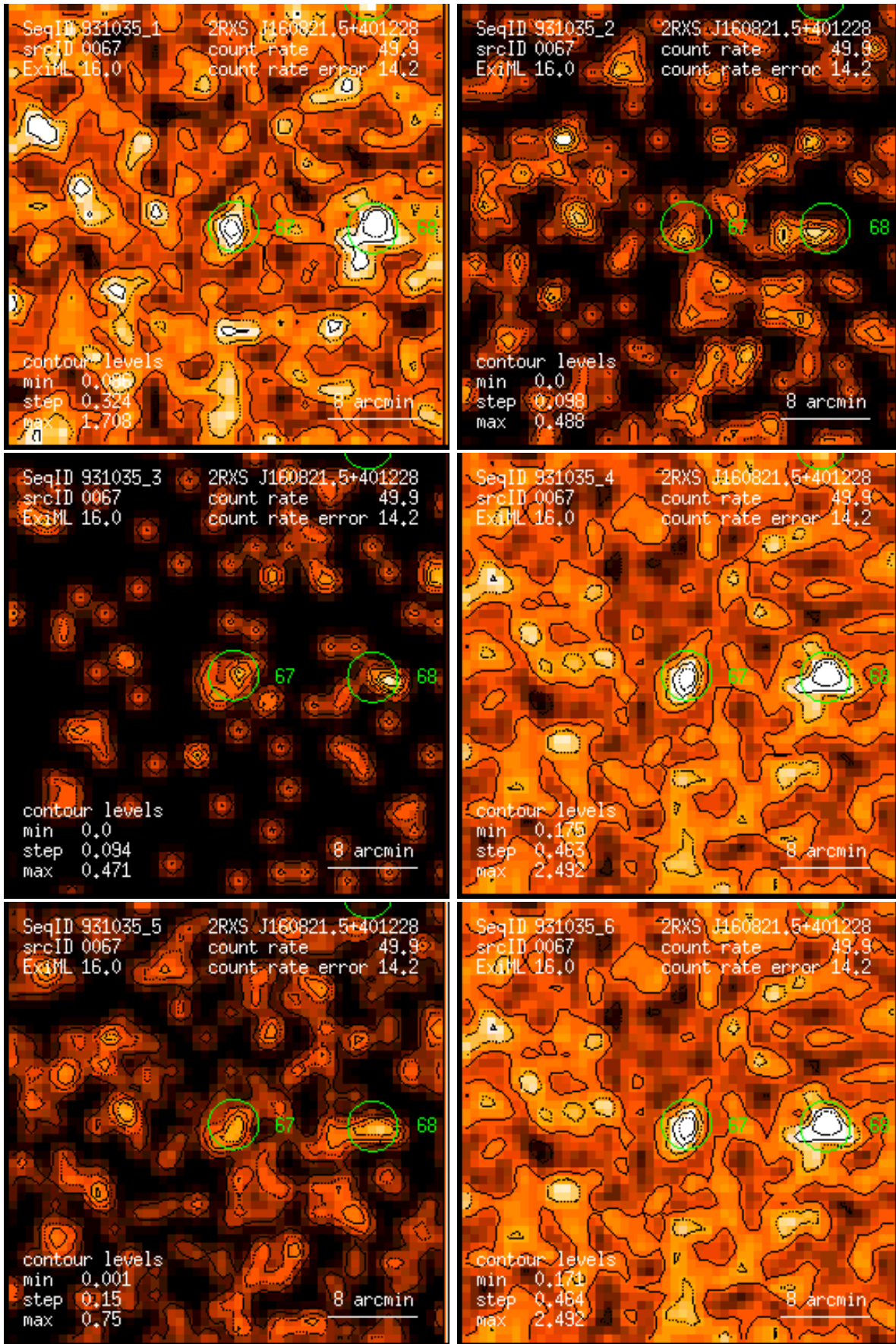
Figure 67: RASS 931035: detection 0067: band rate images, Gaussian filter: (1) PSPC channels 11 – 41, (2) 52 – 90, (3) 91 – 201, (4) 11 – 235, (5) 52 – 201, (6) 11 – 201. Broad band rates in counts/ks. Band rate contour levels in counts/ks/arcmin 2 .
