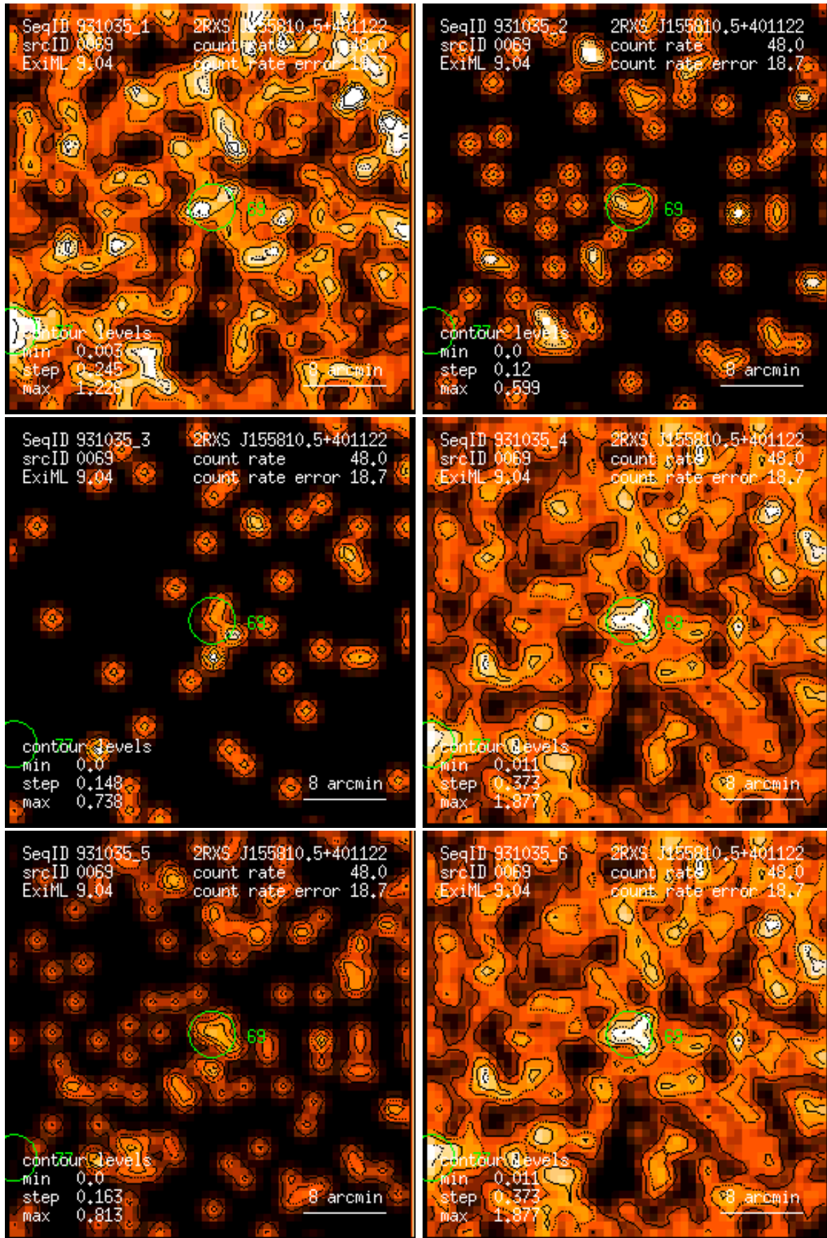
Figure 69: RASS 931035: detection 0069: band rate images, Gaussian filter: (1) PSPC channels 11 – 41, (2) 52 – 90, (3) 91 – 201, (4) 11 – 235, (5) 52 – 201, (6) 11 – 201. Broad band rates in counts/ks. Band rate contour levels in counts/ks/arcmin 2 .
