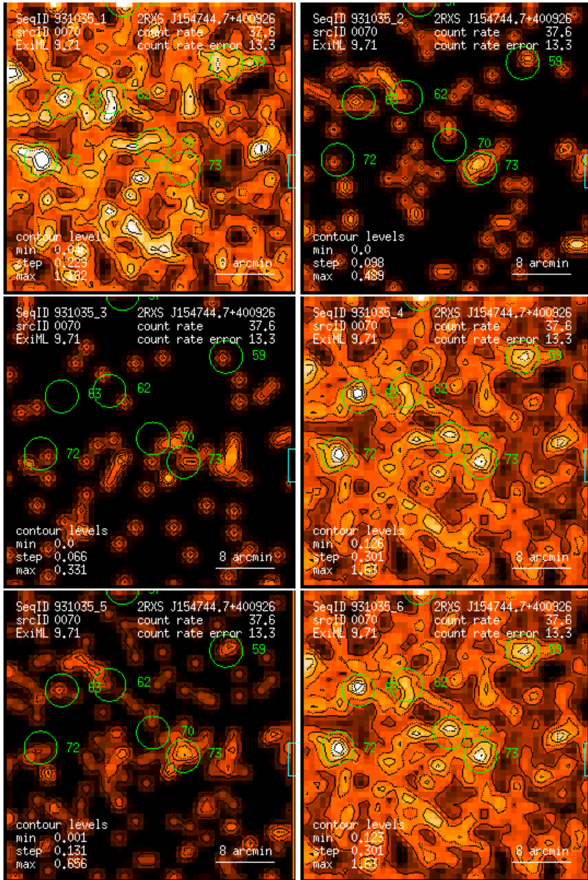
Figure 70: RASS 931035: detection 0070: band rate images, Gaussian filter: (1) PSPC channels 11 – 41, (2) 52 – 90, (3) 91 – 201, (4) 11 – 235, (5) 52 – 201, (6) 11 – 201. Broad band rates in counts/ks. Band rate contour levels in counts/ks/arcmin 2 .
