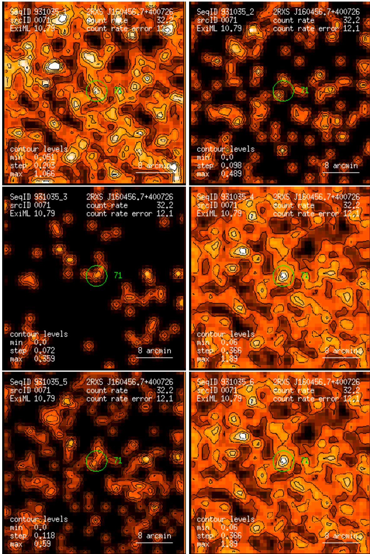
Figure 71: RASS 931035: detection 0071: band rate images, Gaussian filter: (1) PSPC channels 11 – 41, (2) 52 – 90, (3) 91 – 201, (4) 11 – 235, (5) 52 – 201, (6) 11 – 201. Broad band rates in counts/ks. Band rate contour levels in counts/ks/arcmin 2 .
