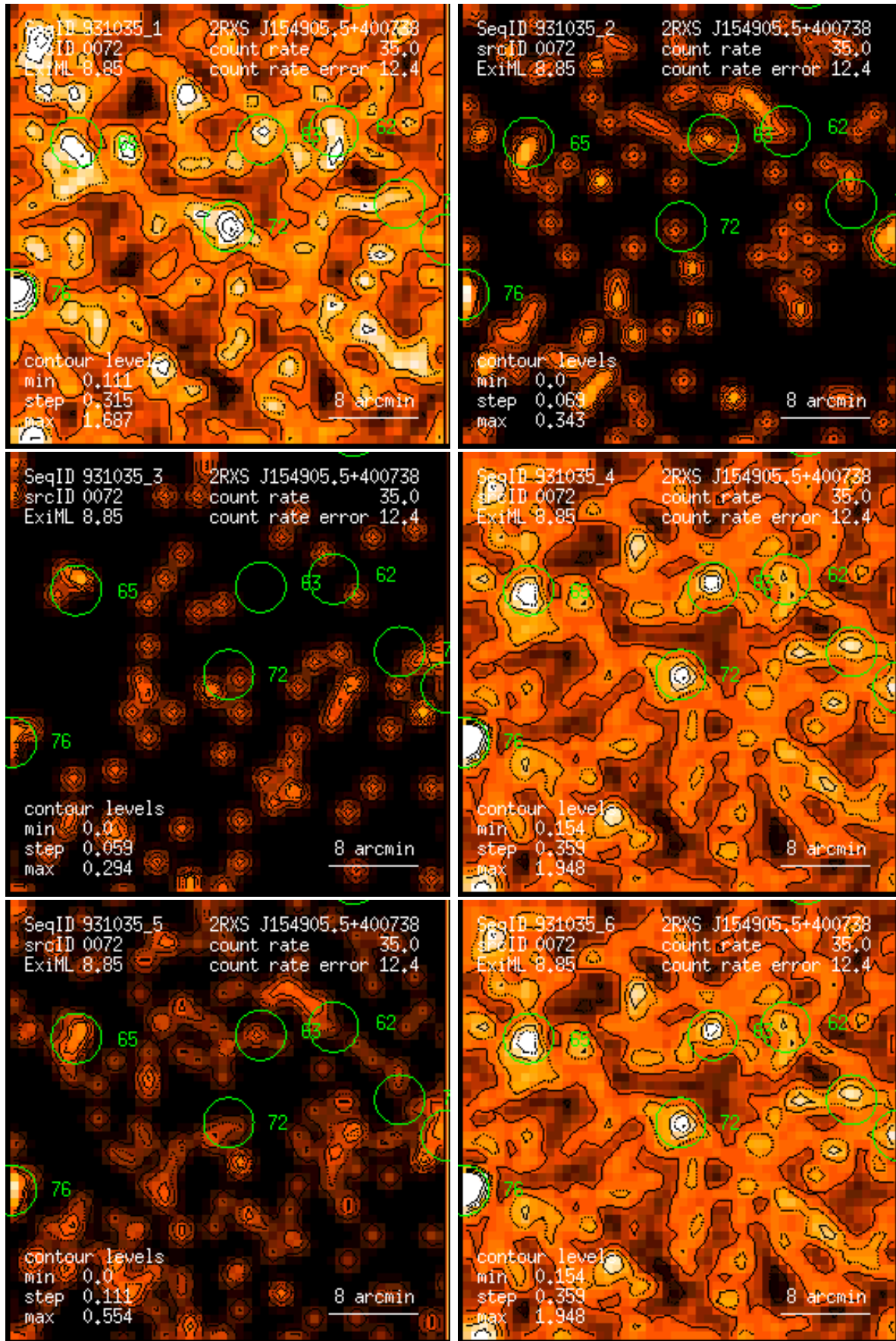
Figure 72: RASS 931035: detection 0072: band rate images, Gaussian filter: (1) PSPC channels 11 – 41, (2) 52 – 90, (3) 91 – 201, (4) 11 – 235, (5) 52 – 201, (6) 11 – 201. Broad band rates in counts/ks. Band rate contour levels in counts/ks/arcmin 2 .
