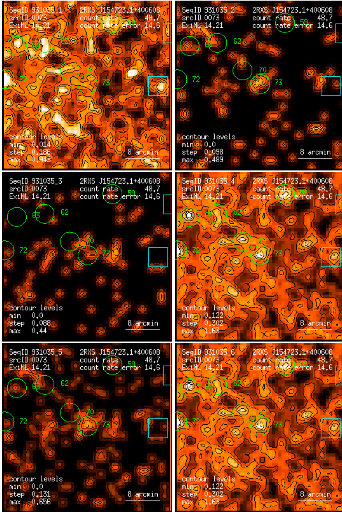
Figure 73: RASS 931035: detection 0073: band rate images, Gaussian filter: (1) PSPC channels 11 – 41, (2) 52 – 90, (3) 91 – 201, (4) 11 – 235, (5) 52 – 201, (6) 11 – 201. Broad band rates in counts/ks. Band rate contour levels in counts/ks/arcmin 2 .
