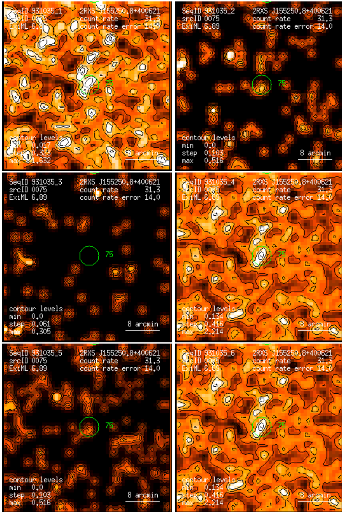
Figure 75: RASS 931035: detection 0075: band rate images, Gaussian filter: (1) PSPC channels 11 – 41, (2) 52 – 90, (3) 91 – 201, (4) 11 – 235, (5) 52 – 201, (6) 11 – 201. Broad band rates in counts/ks. Band rate contour levels in counts/ks/arcmin 2 .
