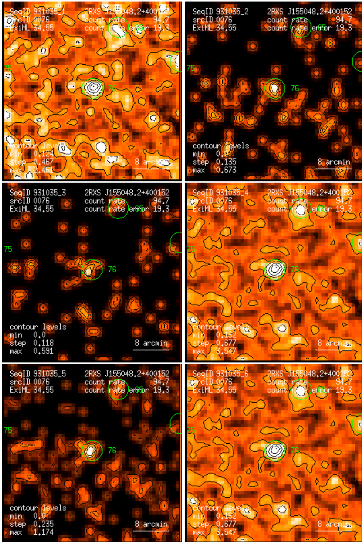
Figure 76: RASS 931035: detection 0076: band rate images, Gaussian filter: (1) PSPC channels 11 – 41, (2) 52 – 90, (3) 91 – 201, (4) 11 – 235, (5) 52 – 201, (6) 11 – 201. Broad band rates in counts/ks. Band rate contour levels in counts/ks/arcmin 2 .
