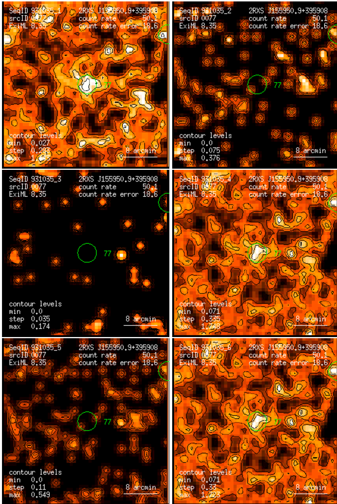
Figure 77: RASS 931035: detection 0077: band rate images, Gaussian filter: (1) PSPC channels 11 – 41, (2) 52 – 90, (3) 91 – 201, (4) 11 – 235, (5) 52 – 201, (6) 11 – 201. Broad band rates in counts/ks. Band rate contour levels in counts/ks/arcmin 2 .
