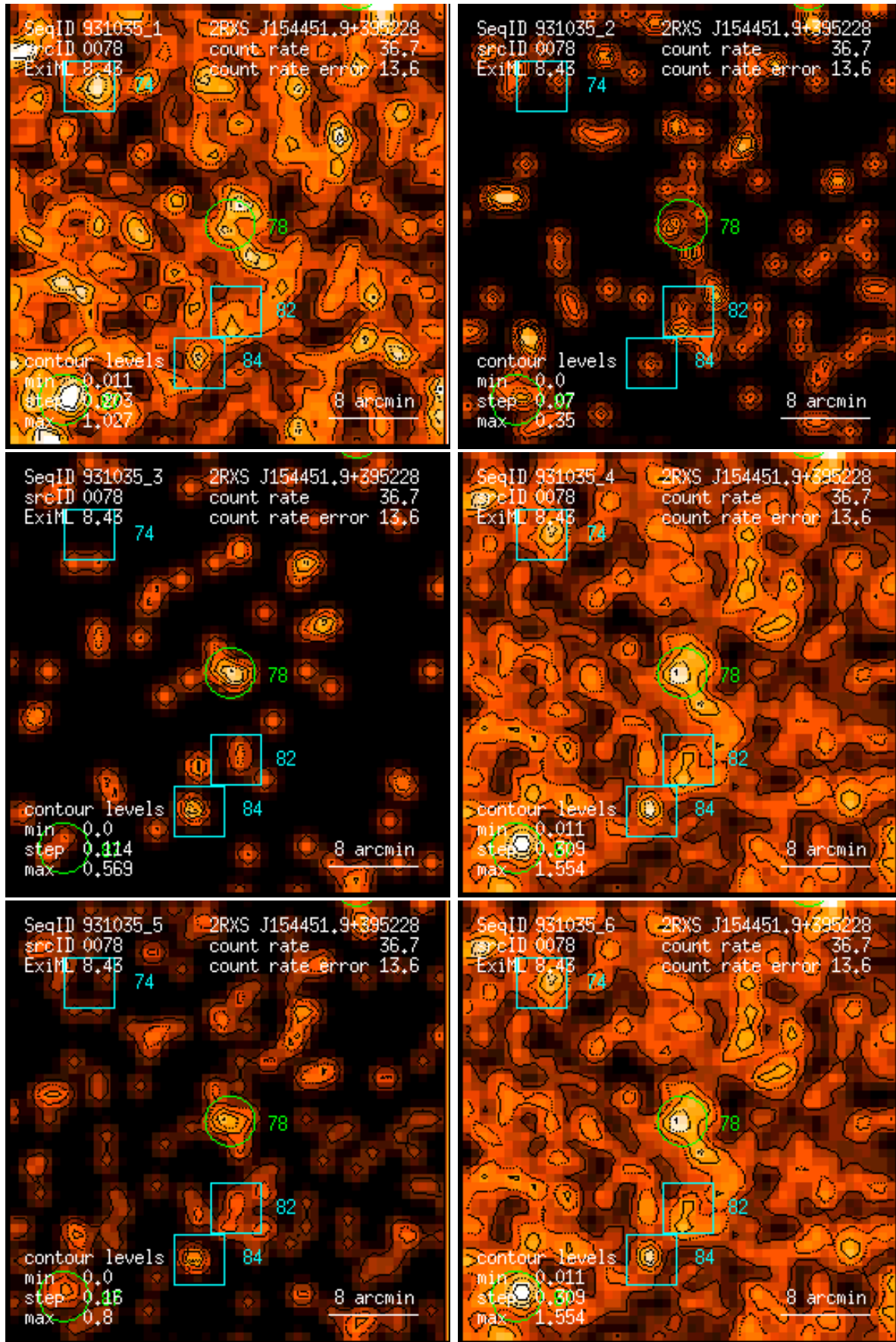
Figure 78: RASS 931035: detection 0078: band rate images, Gaussian filter: (1) PSPC channels 11 – 41, (2) 52 – 90, (3) 91 – 201, (4) 11 – 235, (5) 52 – 201, (6) 11 – 201. Broad band rates in counts/ks. Band rate contour levels in counts/ks/arcmin 2 .
