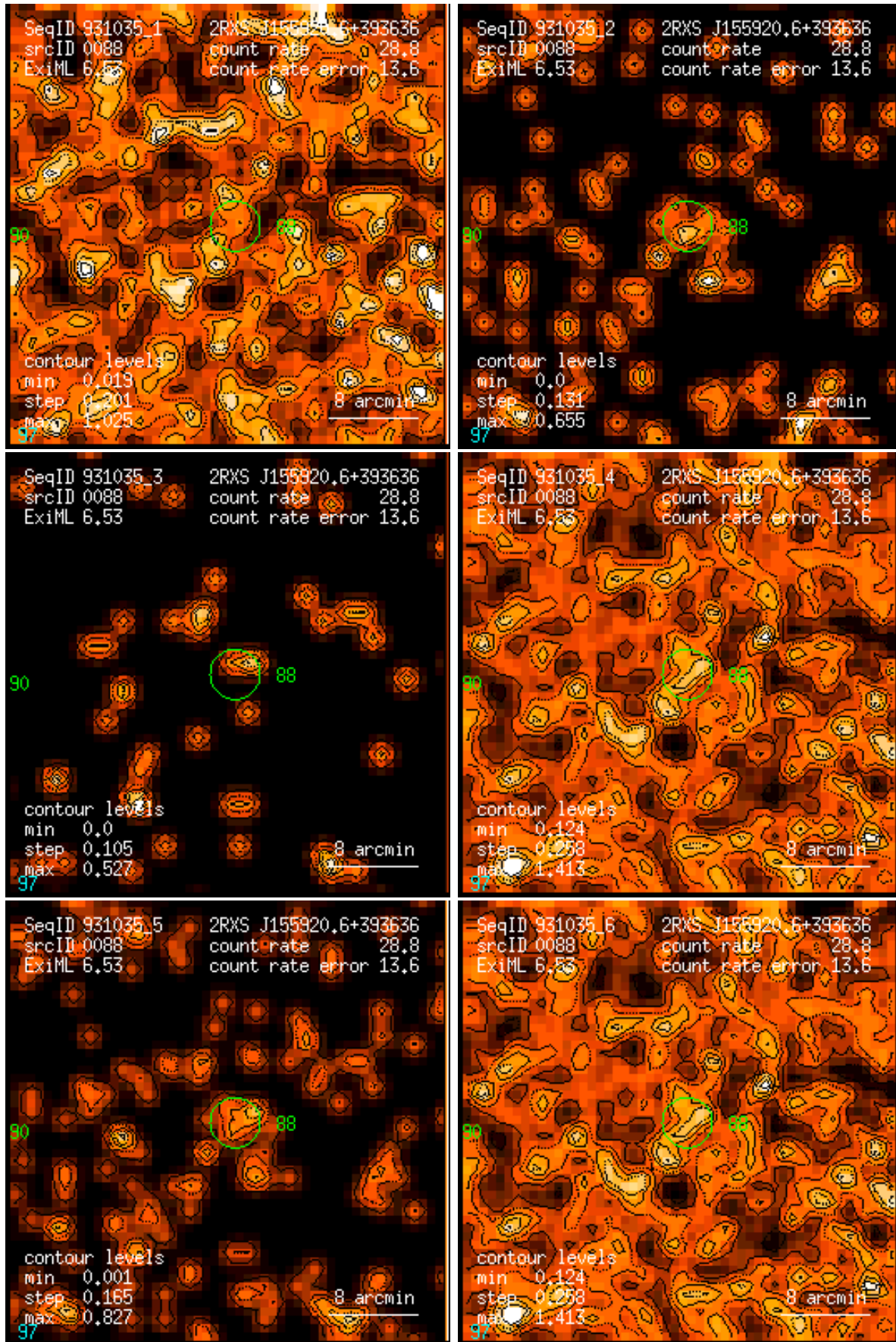
Figure 88: RASS 931035: detection 0088: band rate images, Gaussian filter: (1) PSPC channels 11 – 41, (2) 52 – 90, (3) 91 – 201, (4) 11 – 235, (5) 52 – 201, (6) 11 – 201. Broad band rates in counts/ks. Band rate contour levels in counts/ks/arcmin 2 .
