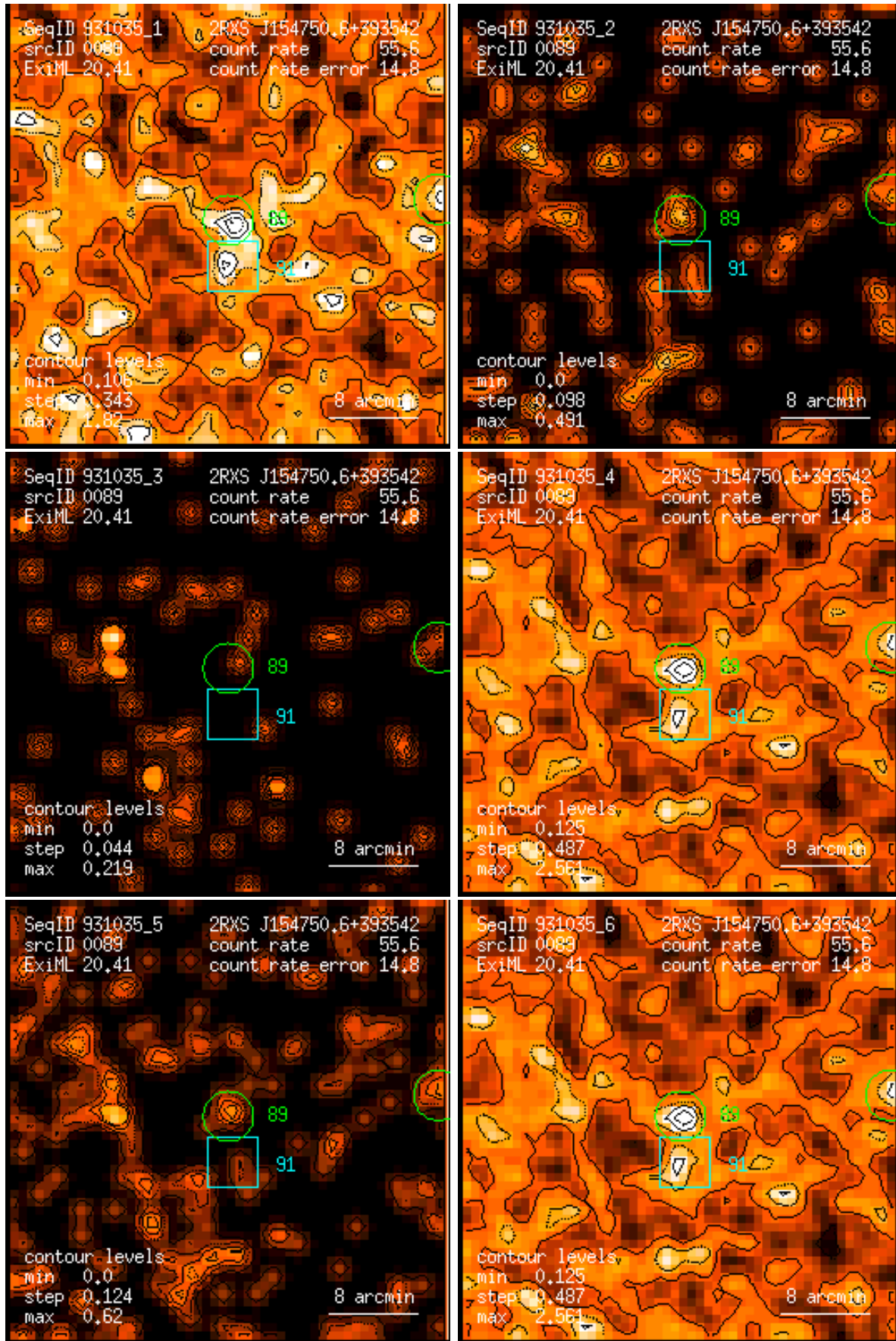
Figure 89: RASS 931035: detection 0089: band rate images, Gaussian filter: (1) PSPC channels 11 – 41, (2) 52 – 90, (3) 91 – 201, (4) 11 – 235, (5) 52 – 201, (6) 11 – 201. Broad band rates in counts/ks. Band rate contour levels in counts/ks/arcmin 2 .
