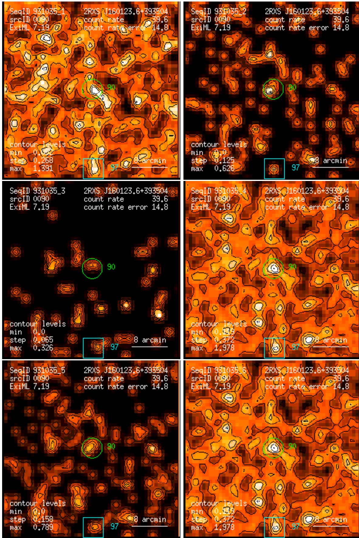
Figure 90: RASS 931035: detection 0090: band rate images, Gaussian filter: (1) PSPC channels 11 – 41, (2) 52 – 90, (3) 91 – 201, (4) 11 – 235, (5) 52 – 201, (6) 11 – 201. Broad band rates in counts/ks. Band rate contour levels in counts/ks/arcmin 2 .
