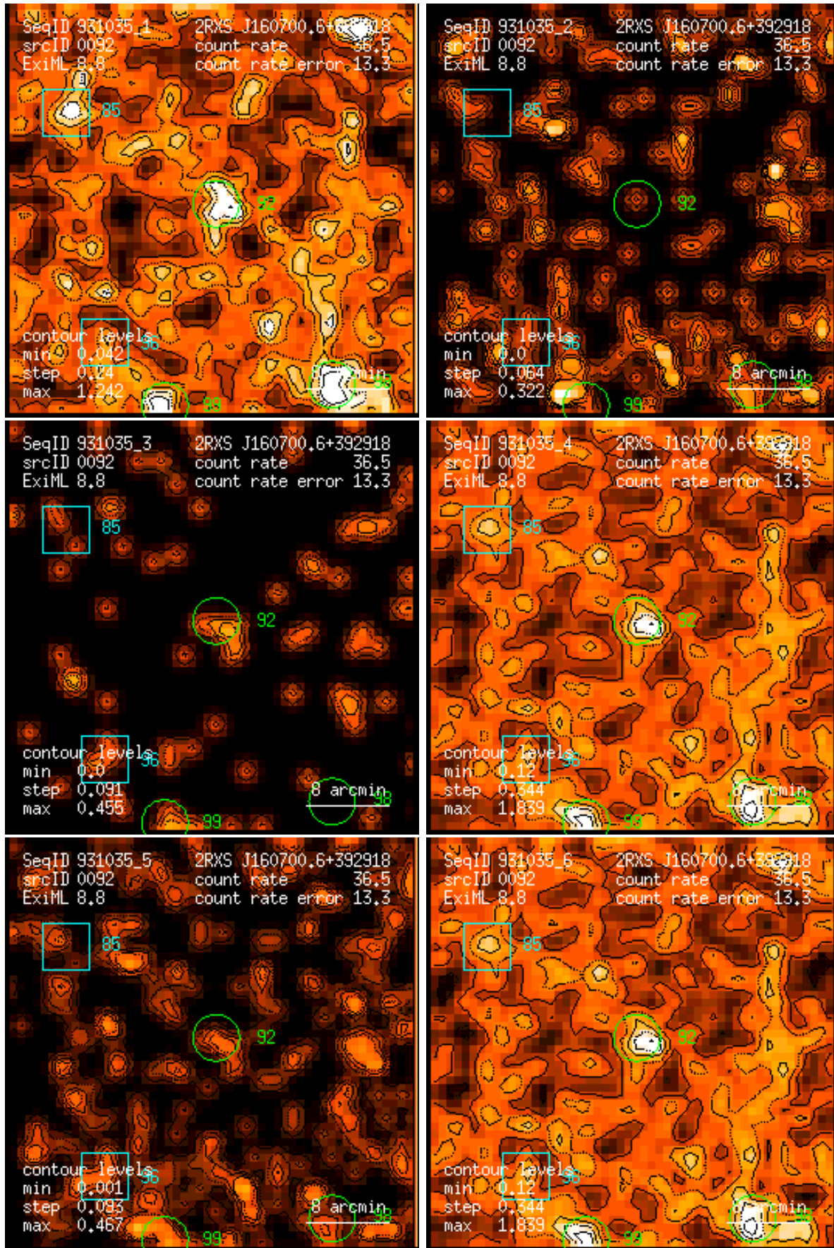
Figure 92: RASS 931035: detection 0092: band rate images, Gaussian filter: (1) PSPC channels 11 – 41, (2) 52 – 90, (3) 91 – 201, (4) 11 – 235, (5) 52 – 201, (6) 11 – 201. Broad band rates in counts/ks. Band rate contour levels in counts/ks/arcmin 2 .
