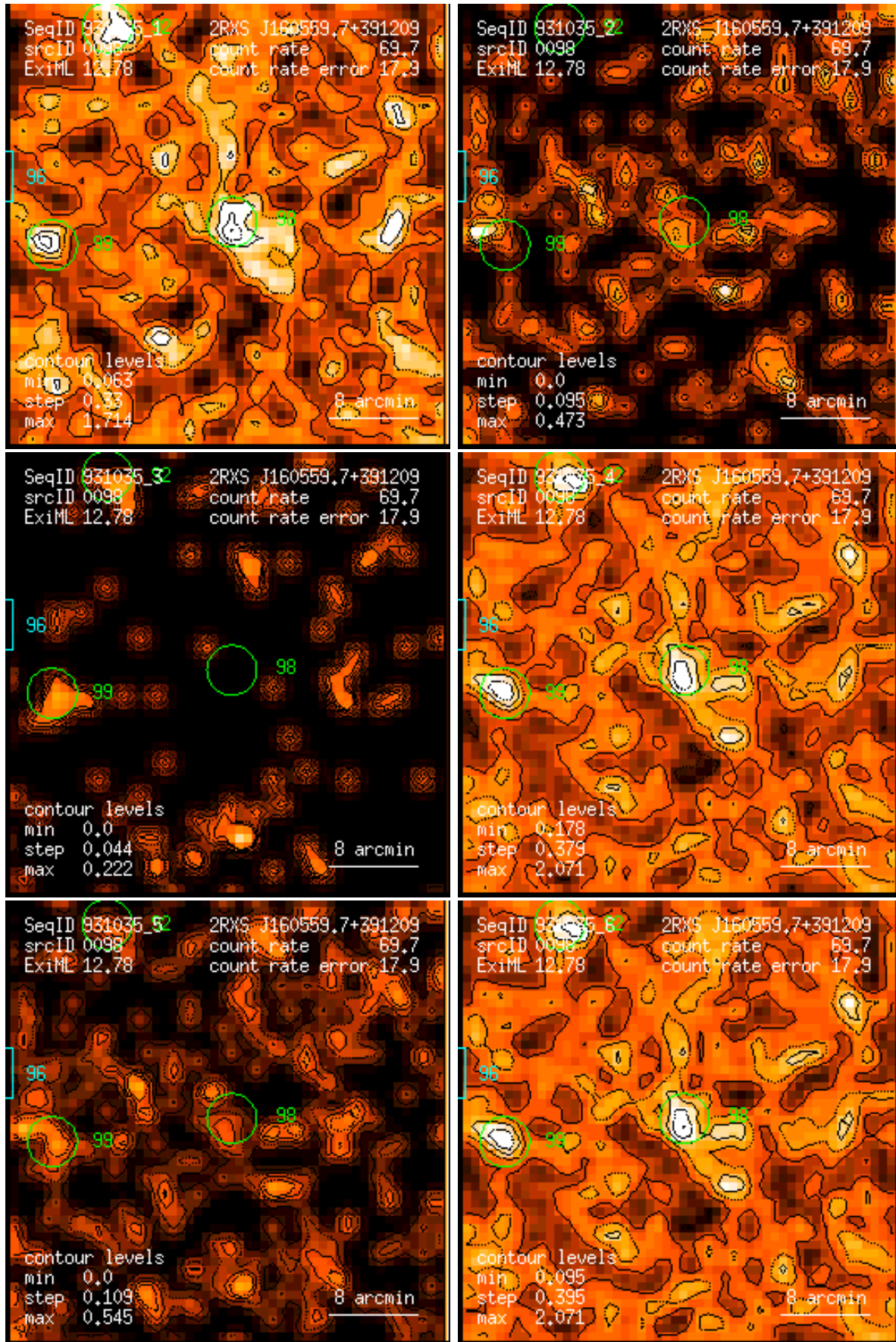
Figure 98: RASS 931035: detection 0098: band rate images, Gaussian filter: (1) PSPC channels 11 – 41, (2) 52 – 90, (3) 91 – 201, (4) 11 – 235, (5) 52 – 201, (6) 11 – 201. Broad band rates in counts/ks. Band rate contour levels in counts/ks/arcmin 2 .
