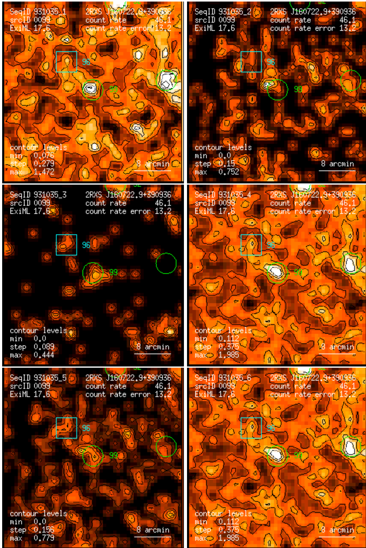
Figure 99: RASS 931035: detection 0099: band rate images, Gaussian filter: (1) PSPC channels 11 – 41, (2) 52 – 90, (3) 91 – 201, (4) 11 – 235, (5) 52 – 201, (6) 11 – 201. Broad band rates in counts/ks. Band rate contour levels in counts/ks/arcmin 2 .
