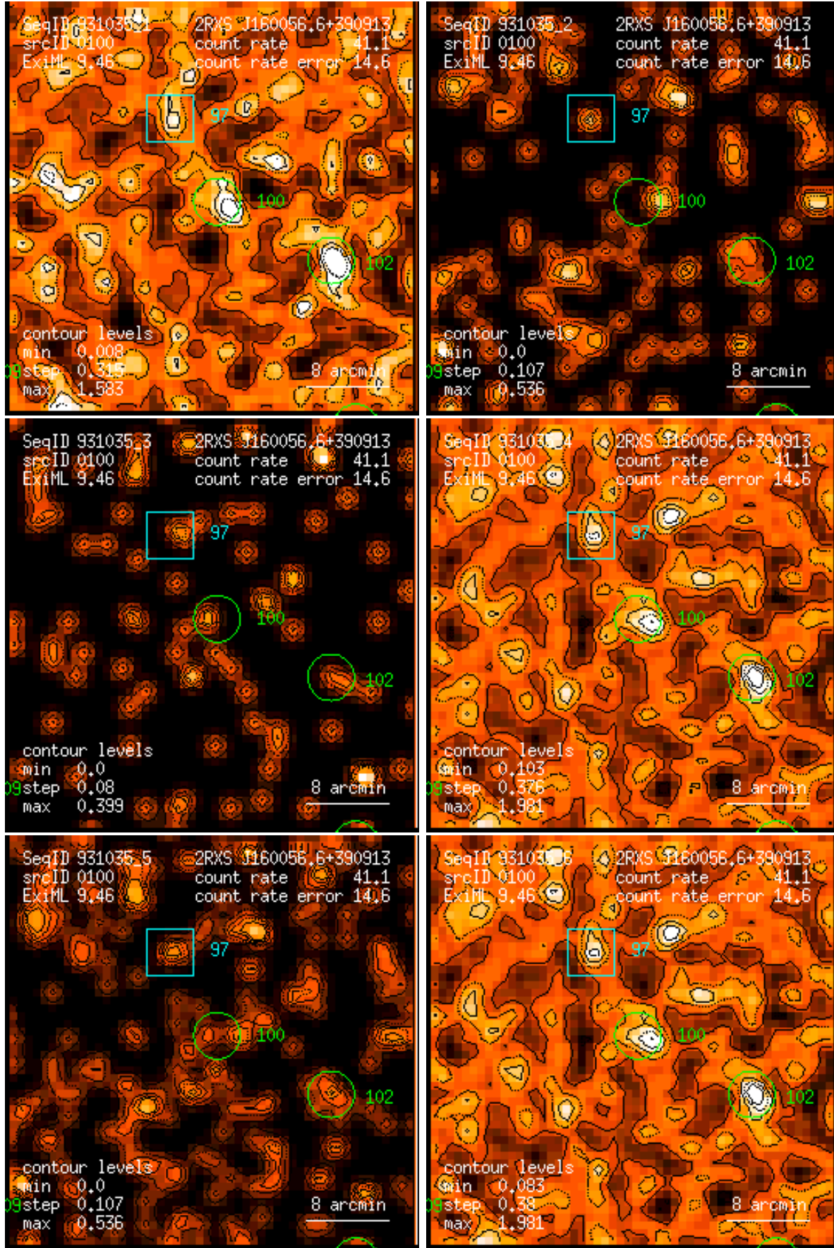
Figure 100: RASS 931035: detection 0100: band rate images, Gaussian filter: (1) PSPC channels 11 – 41, (2) 52 – 90, (3) 91 – 201, (4) 11 – 235, (5) 52 – 201, (6) 11 – 201. Broad band rates in counts/ks. Band rate contour levels in counts/ks/arcmin 2 .
