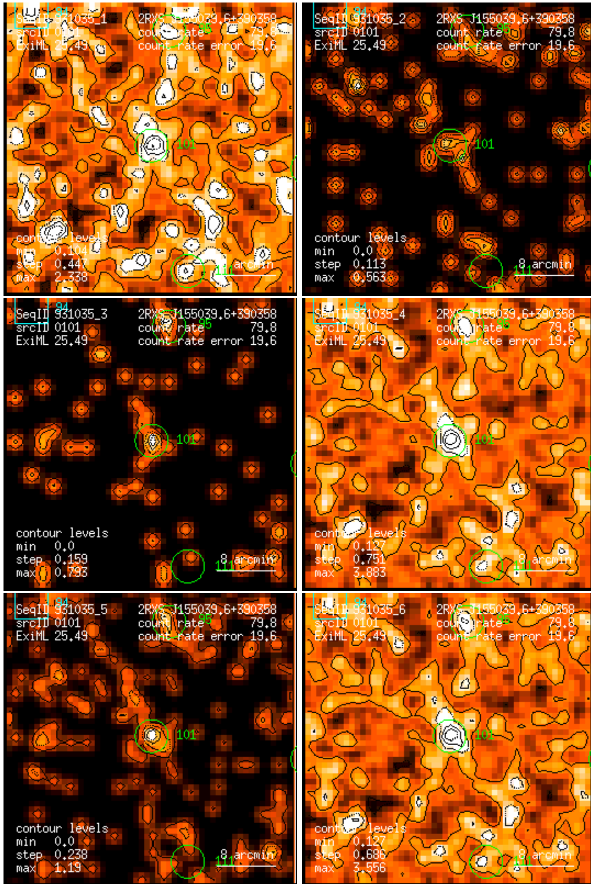
Figure 101: RASS 931035: detection 0101: band rate images, Gaussian filter: (1) PSPC channels 11 – 41, (2) 52 – 90, (3) 91 – 201, (4) 11 – 235, (5) 52 – 201, (6) 11 – 201. Broad band rates in counts/ks. Band rate contour levels in counts/ks/arcmin 2 .
