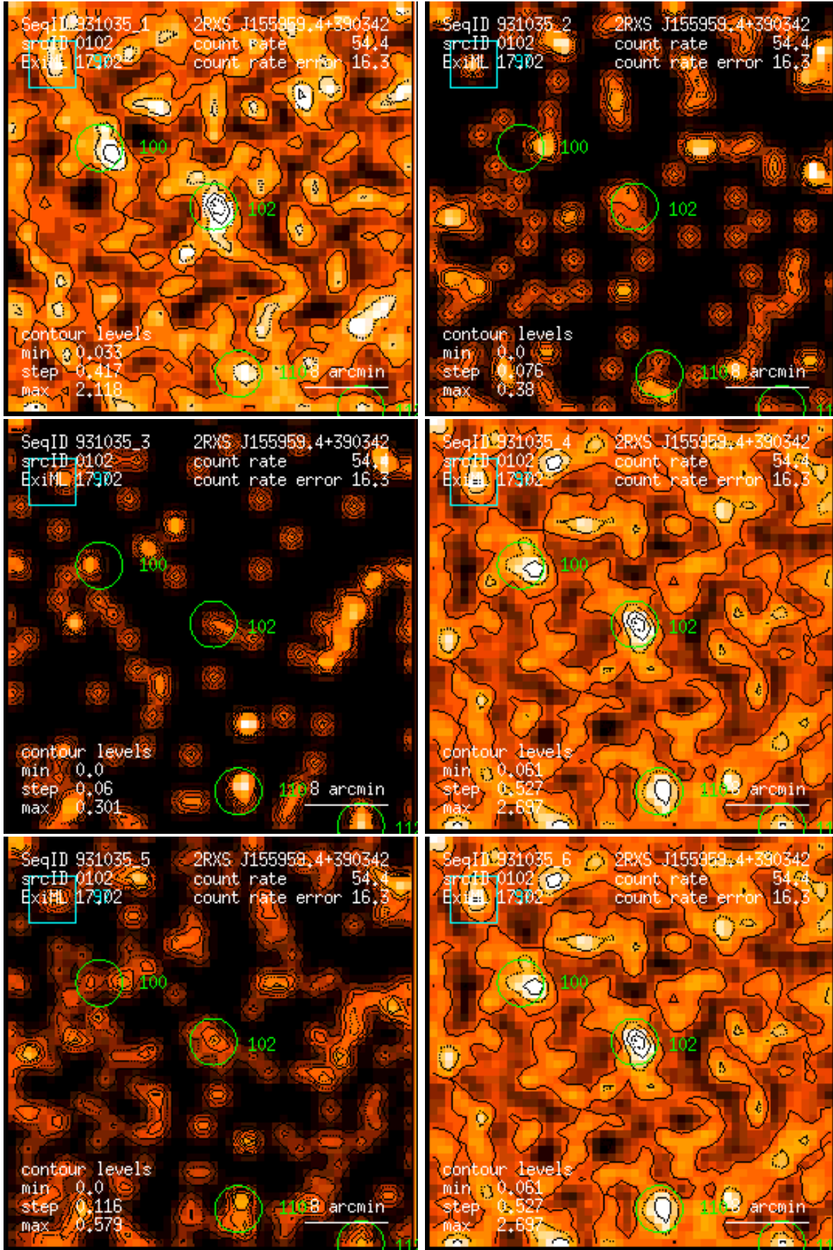
Figure 102: RASS 931035: detection 0102: band rate images, Gaussian filter: (1) PSPC channels 11 – 41, (2) 52 – 90, (3) 91 – 201, (4) 11 – 235, (5) 52 – 201, (6) 11 – 201. Broad band rates in counts/ks. Band rate contour levels in counts/ks/arcmin 2 .
