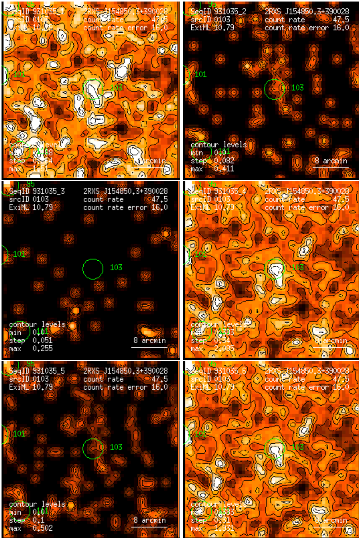
Figure 103: RASS 931035: detection 0103: band rate images, Gaussian filter: (1) PSPC channels 11 – 41, (2) 52 – 90, (3) 91 – 201, (4) 11 – 235, (5) 52 – 201, (6) 11 – 201. Broad band rates in counts/ks. Band rate contour levels in counts/ks/arcmin 2 .
