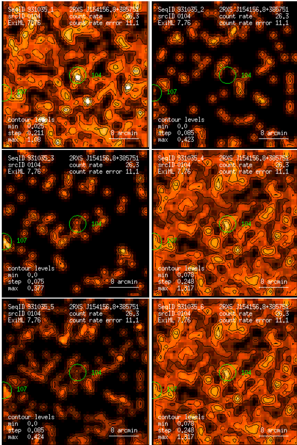
Figure 104: RASS 931035: detection 0104: band rate images, Gaussian filter: (1) PSPC channels 11 – 41, (2) 52 – 90, (3) 91 – 201, (4) 11 – 235, (5) 52 – 201, (6) 11 – 201. Broad band rates in counts/ks. Band rate contour levels in counts/ks/arcmin 2 .
