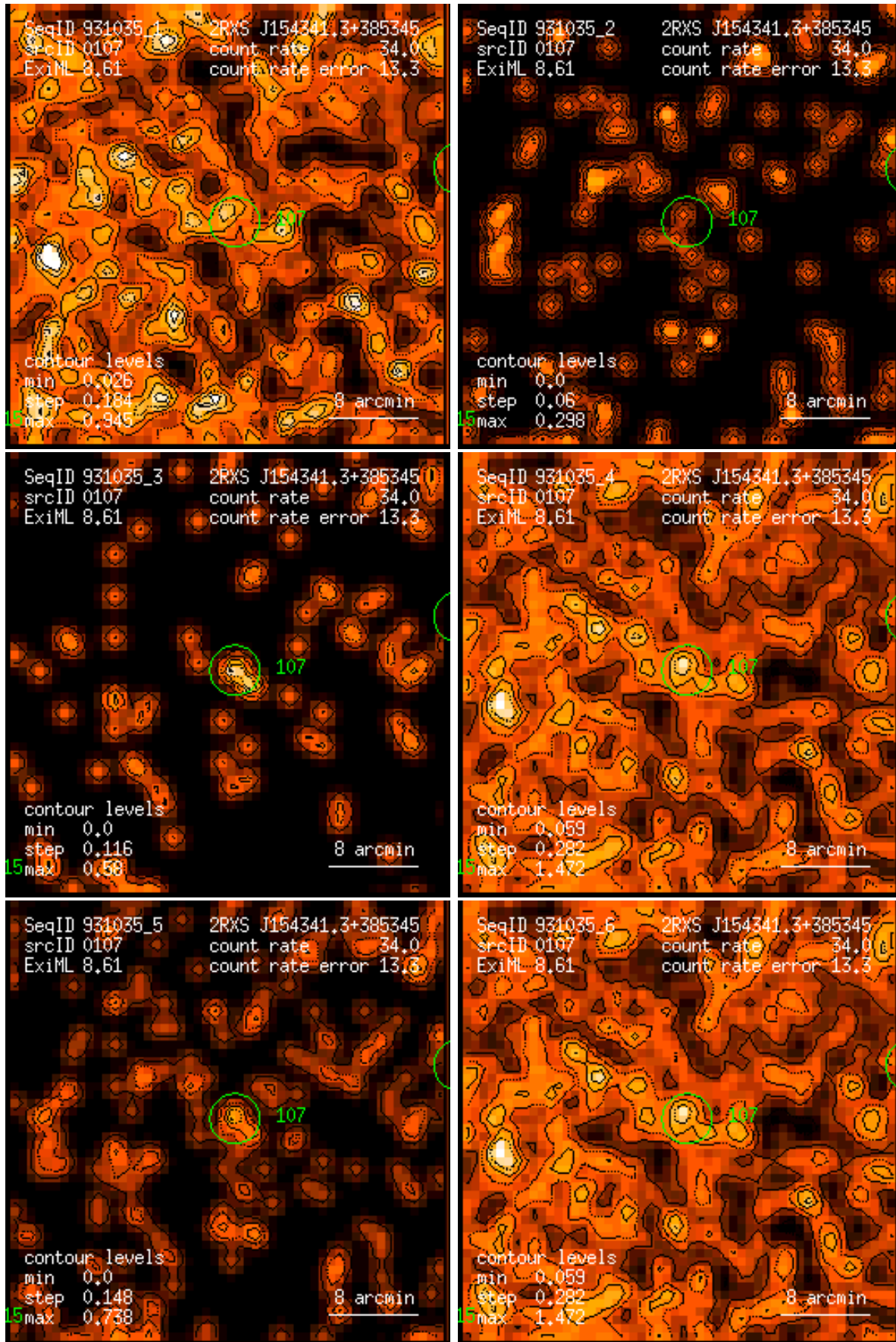
Figure 107: RASS 931035: detection 0107: band rate images, Gaussian filter: (1) PSPC channels 11 – 41, (2) 52 – 90, (3) 91 – 201, (4) 11 – 235, (5) 52 – 201, (6) 11 – 201. Broad band rates in counts/ks. Band rate contour levels in counts/ks/arcmin 2 .
