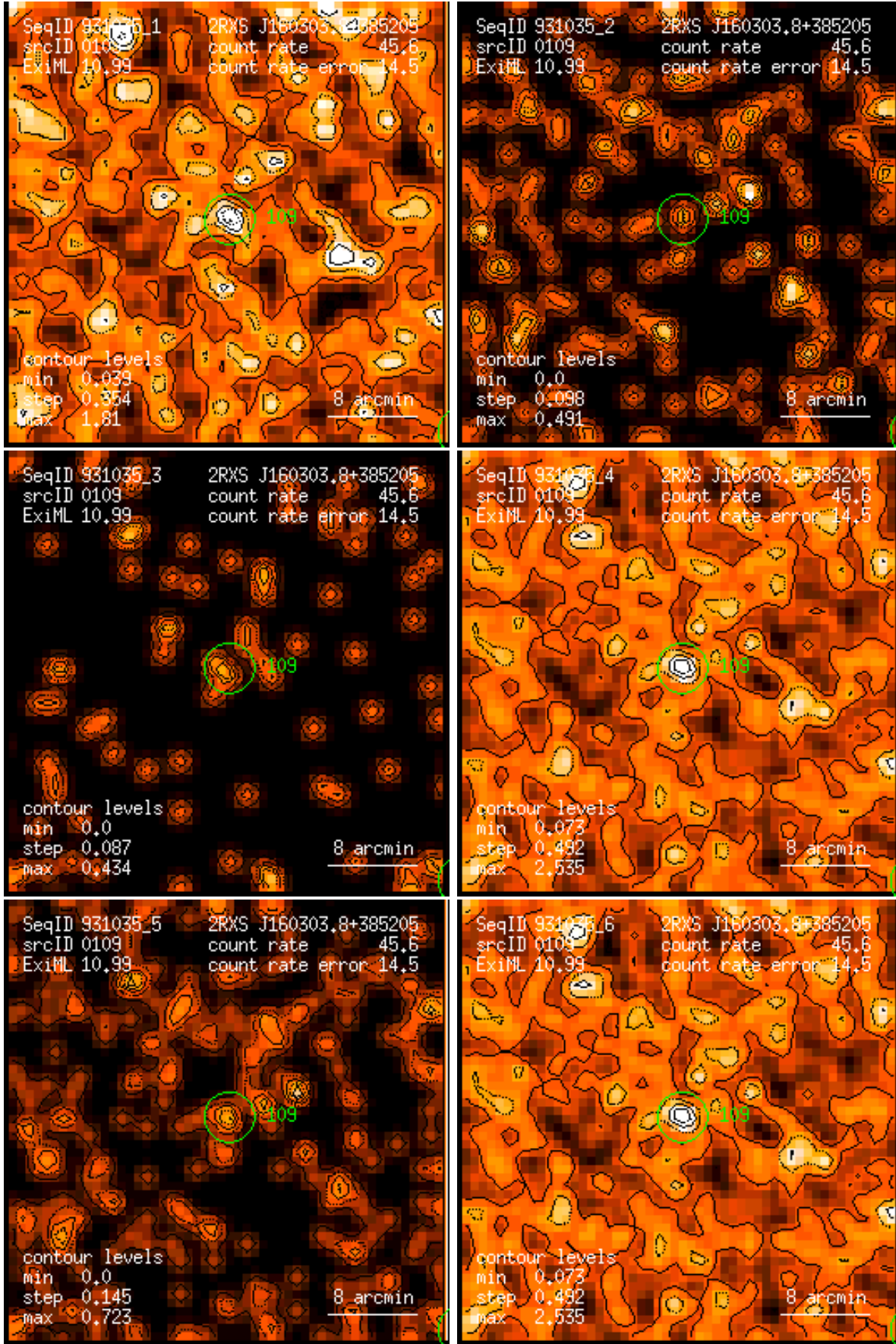
Figure 109: RASS 931035: detection 0109: band rate images, Gaussian filter: (1) PSPC channels 11 – 41, (2) 52 – 90, (3) 91 – 201, (4) 11 – 235, (5) 52 – 201, (6) 11 – 201. Broad band rates in counts/ks. Band rate contour levels in counts/ks/arcmin 2 .
