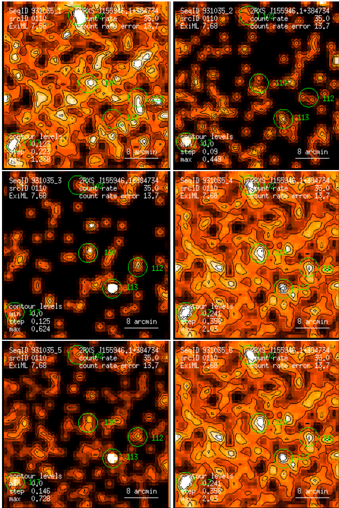
Figure 110: RASS 931035: detection 0110: band rate images, Gaussian filter: (1) PSPC channels 11 – 41, (2) 52 – 90, (3) 91 – 201, (4) 11 – 235, (5) 52 – 201, (6) 11 – 201. Broad band rates in counts/ks. Band rate contour levels in counts/ks/arcmin 2 .
