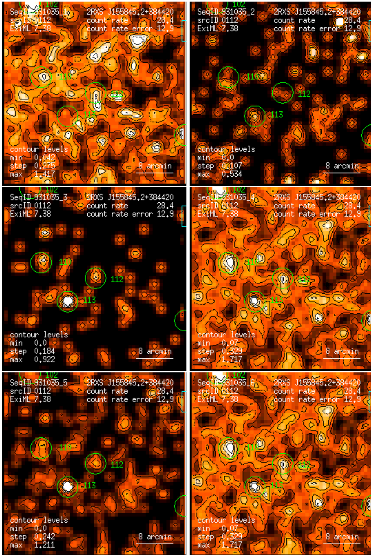
Figure 112: RASS 931035: detection 0112: band rate images, Gaussian filter: (1) PSPC channels 11 – 41, (2) 52 – 90, (3) 91 – 201, (4) 11 – 235, (5) 52 – 201, (6) 11 – 201. Broad band rates in counts/ks. Band rate contour levels in counts/ks/arcmin 2 .
